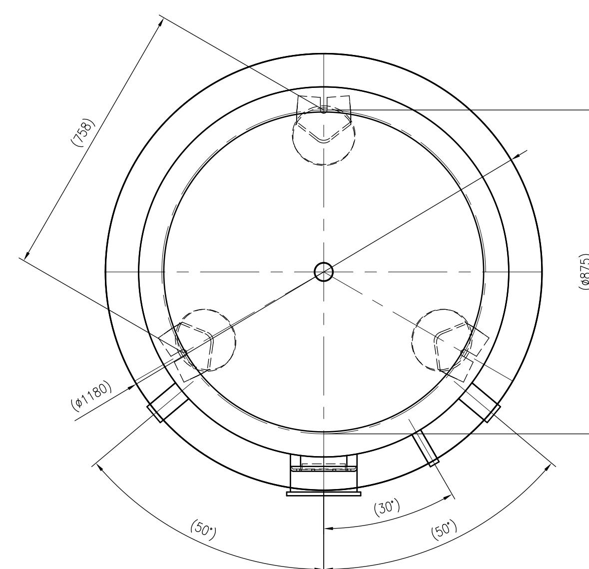
Top view
