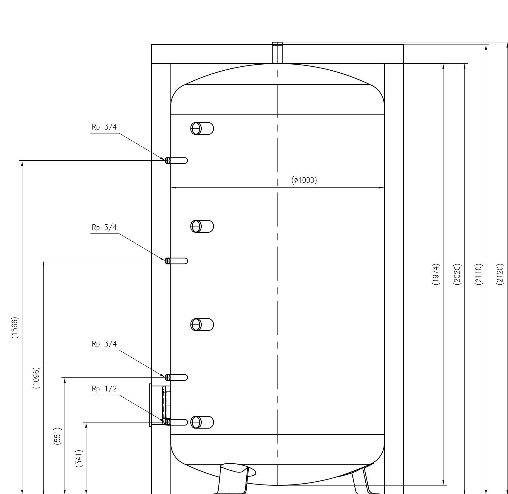
Side view
