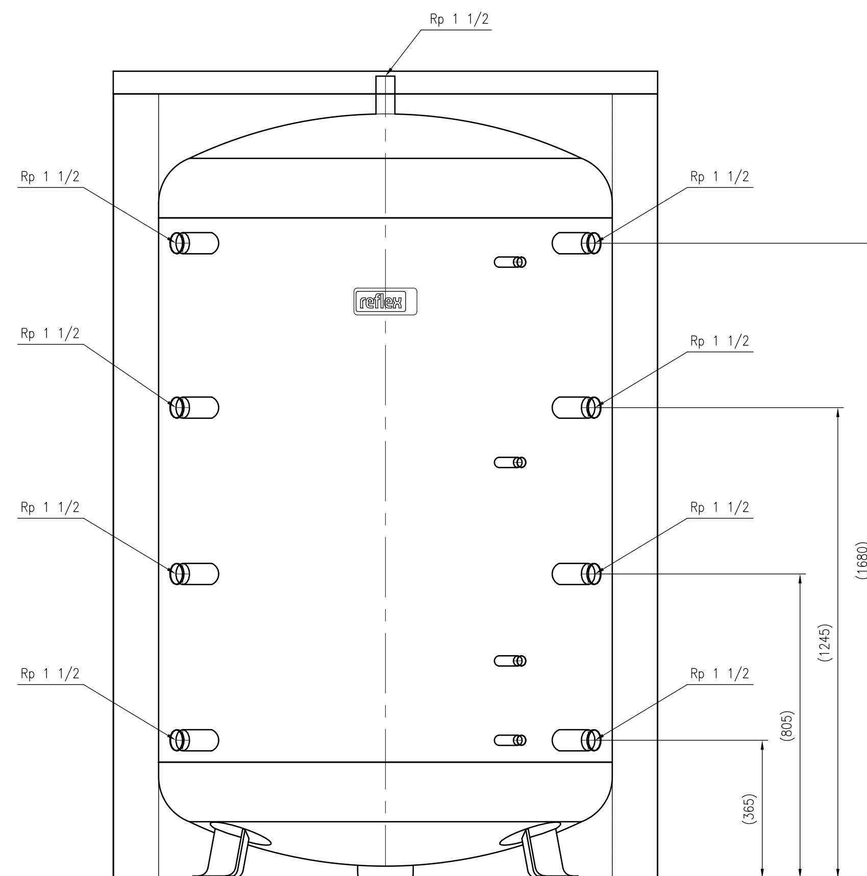
Front view
