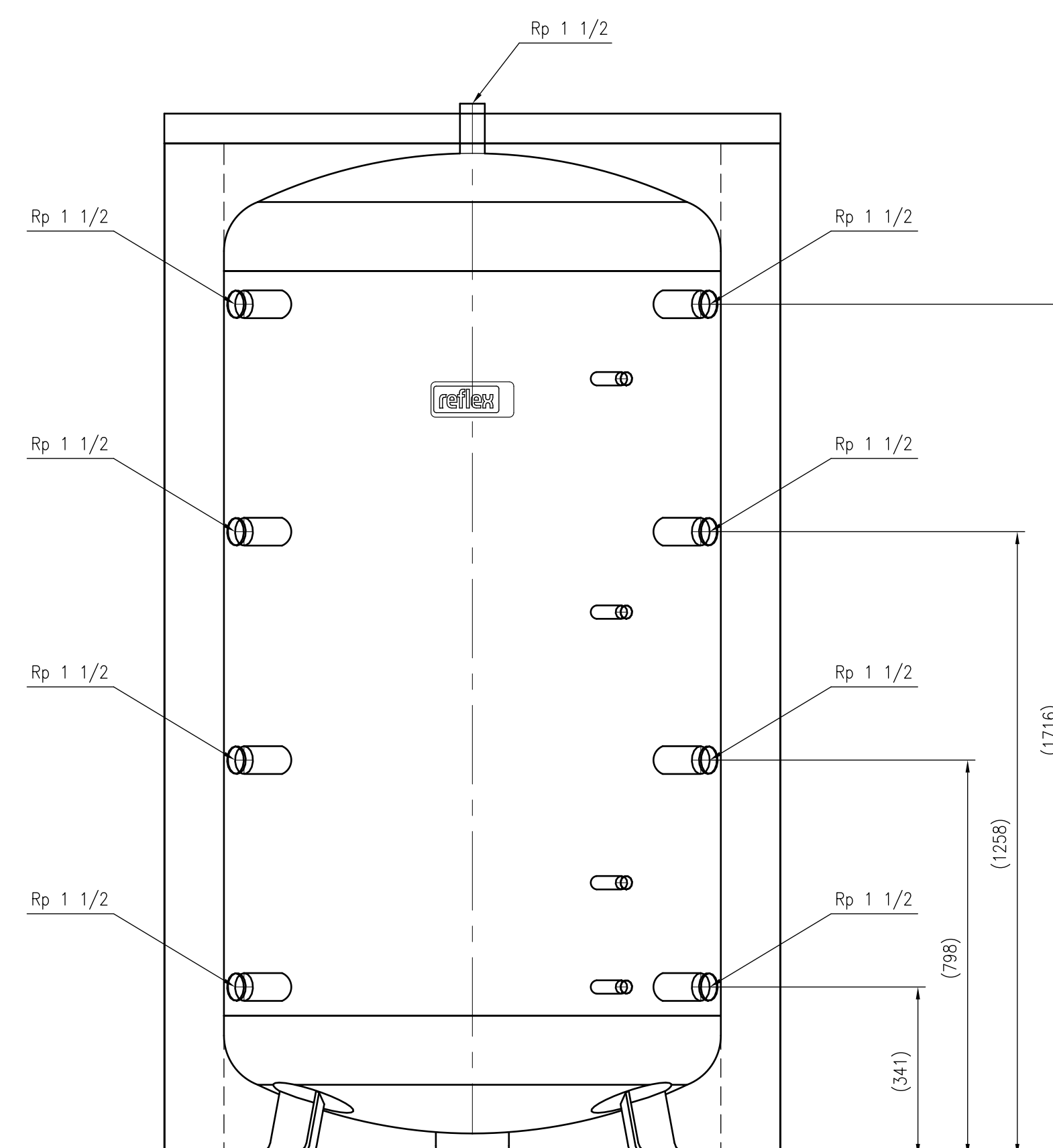
Front view
