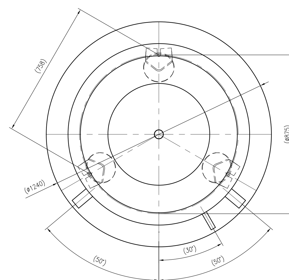
Top view
