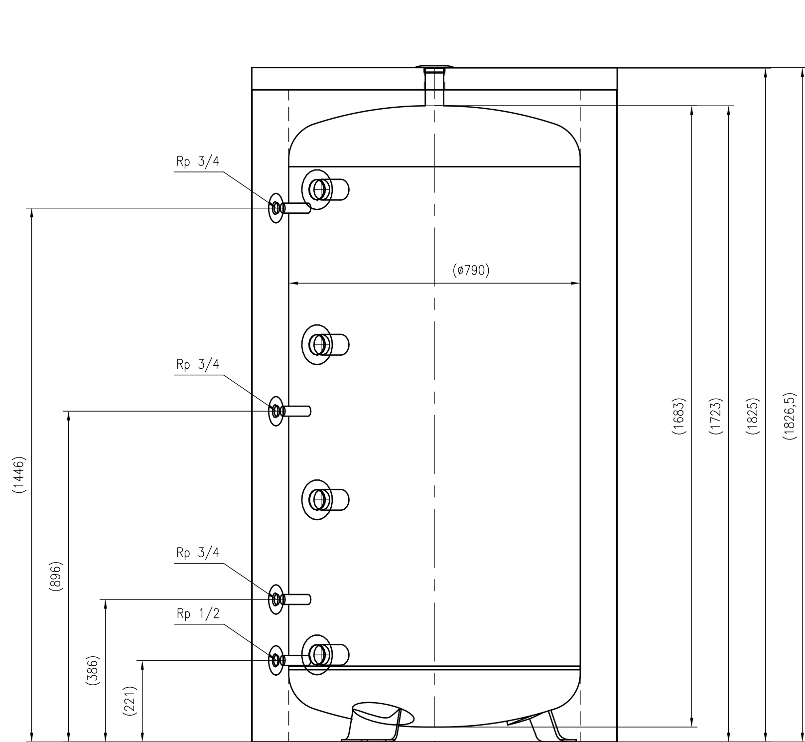
Side view
