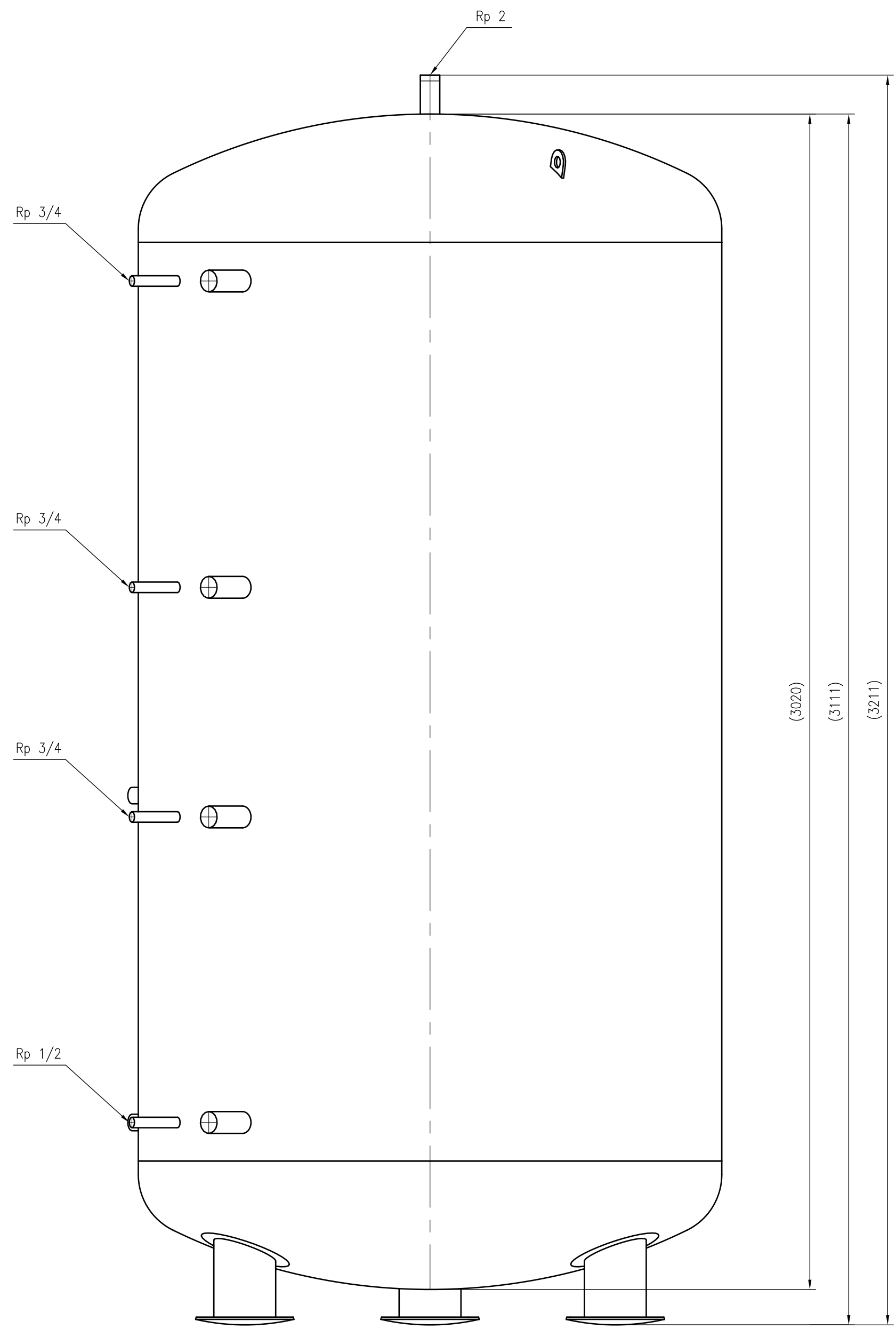
Side view
