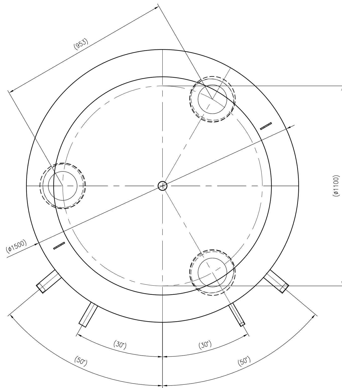
Top view
