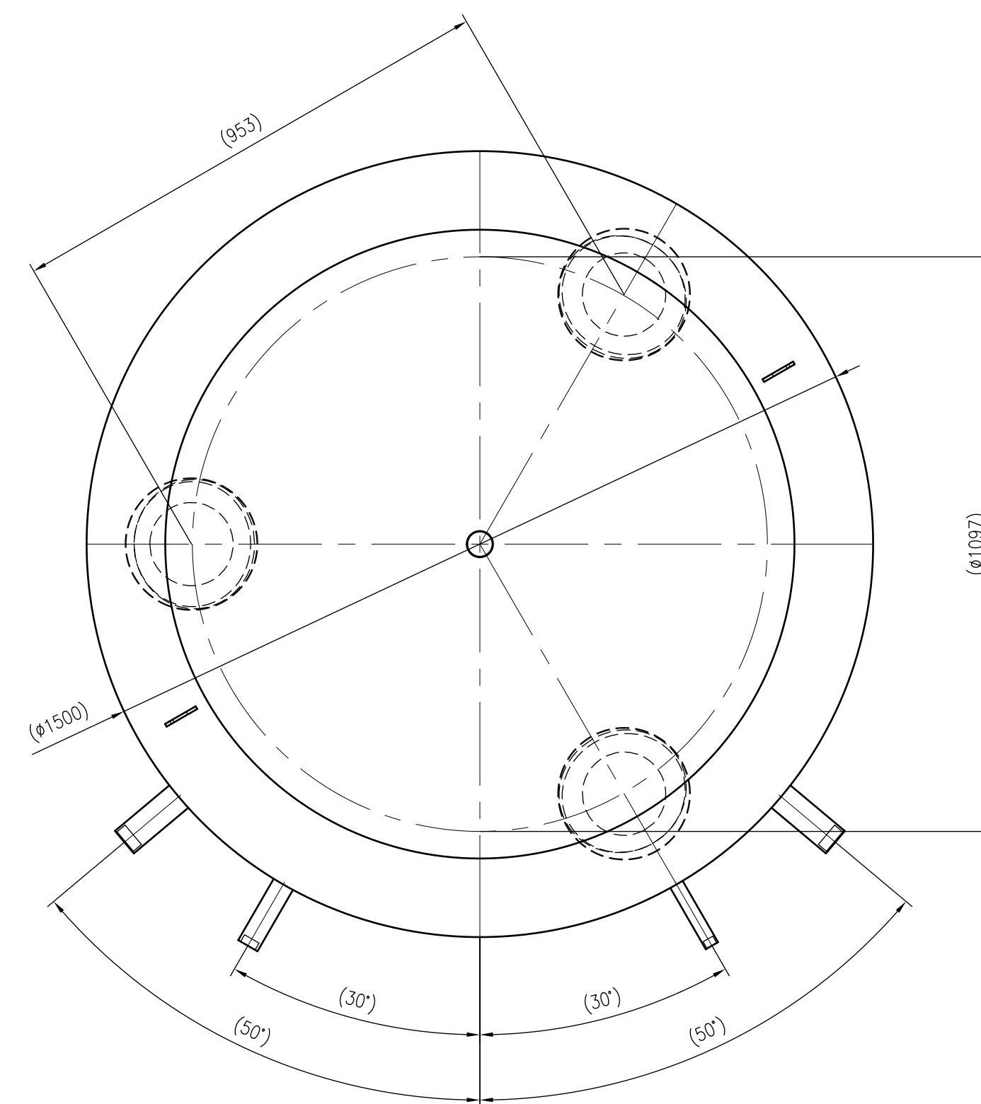
Top view
