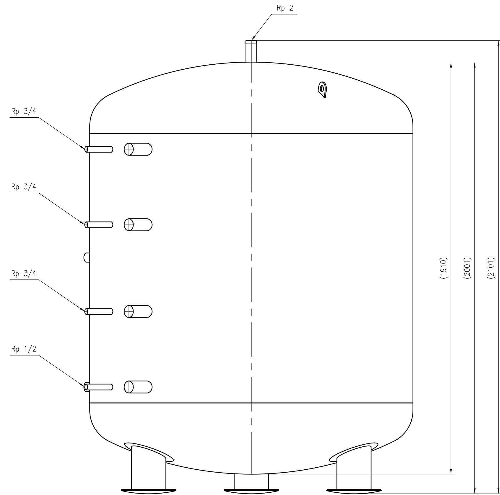
Side view
