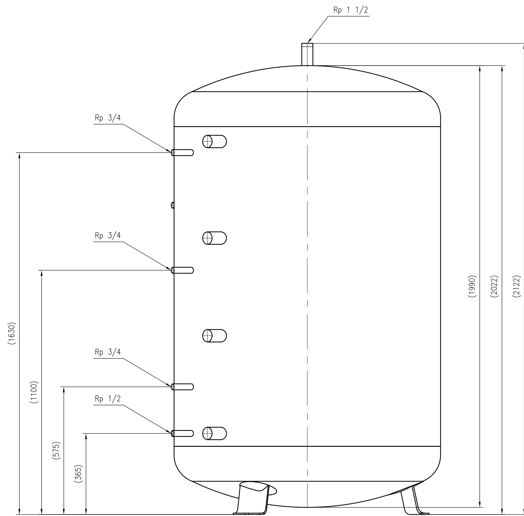
Side view
