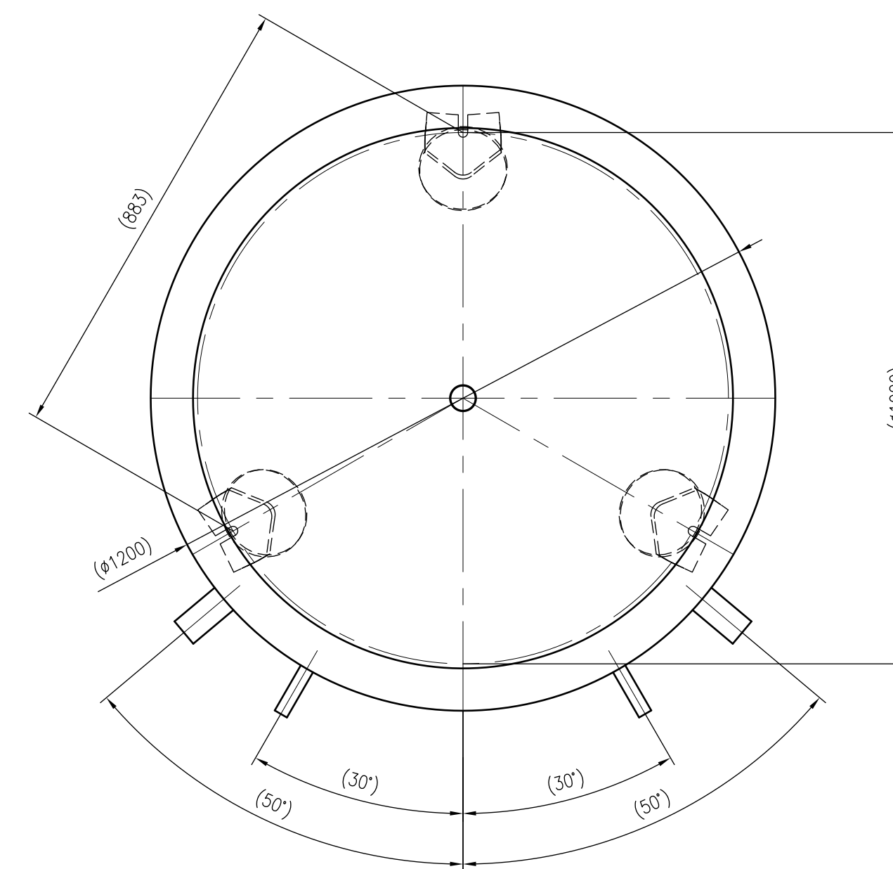
Top view
