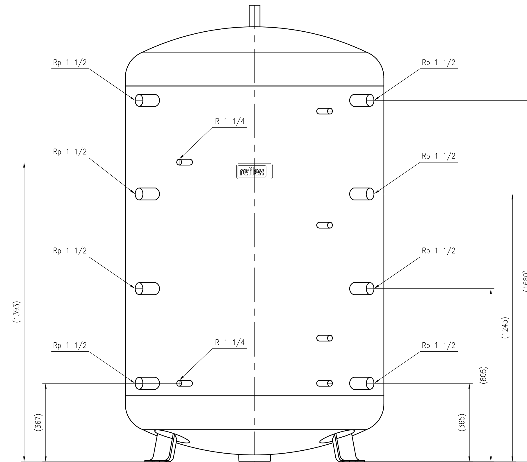
Front view
