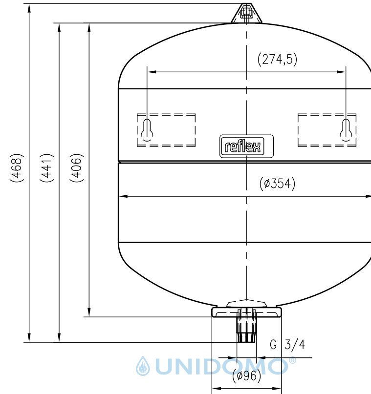
Front view
