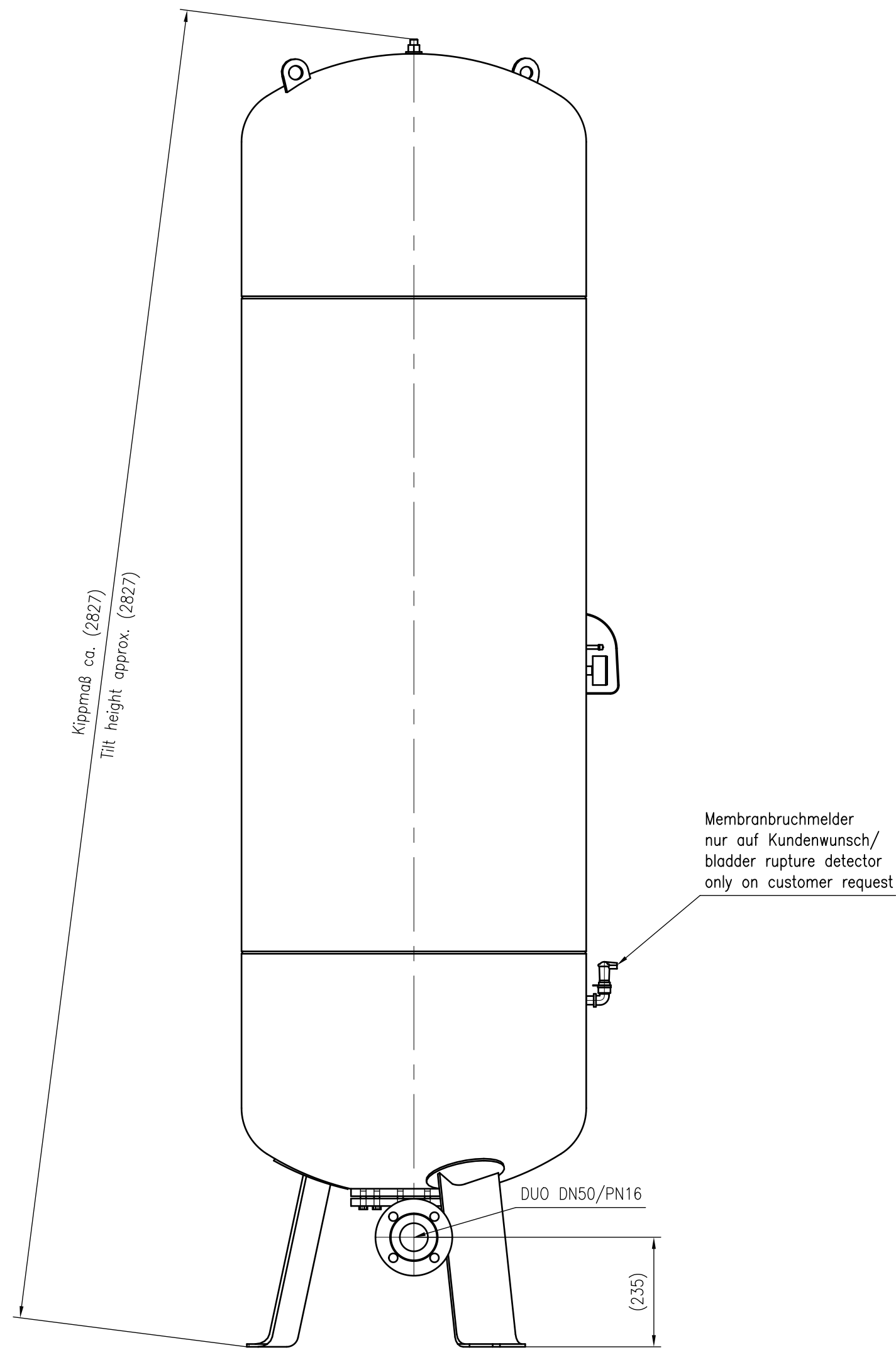
Side view
