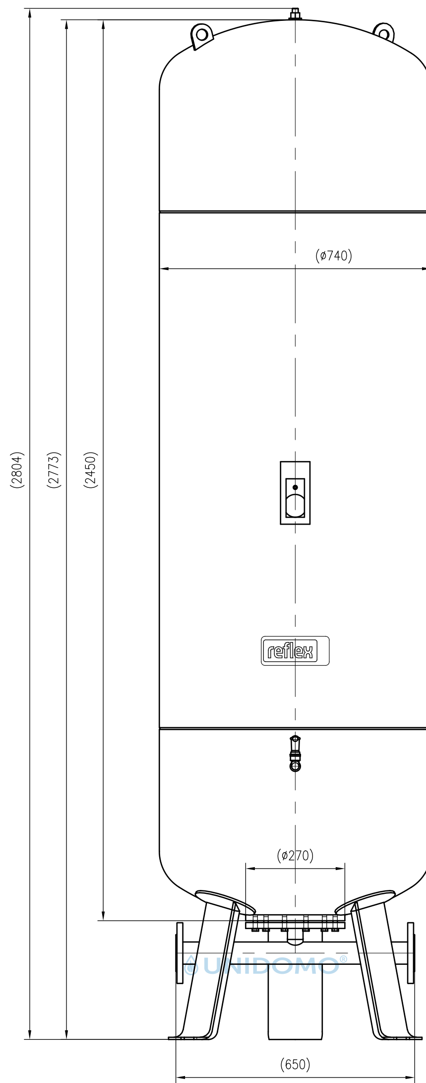
Front view
