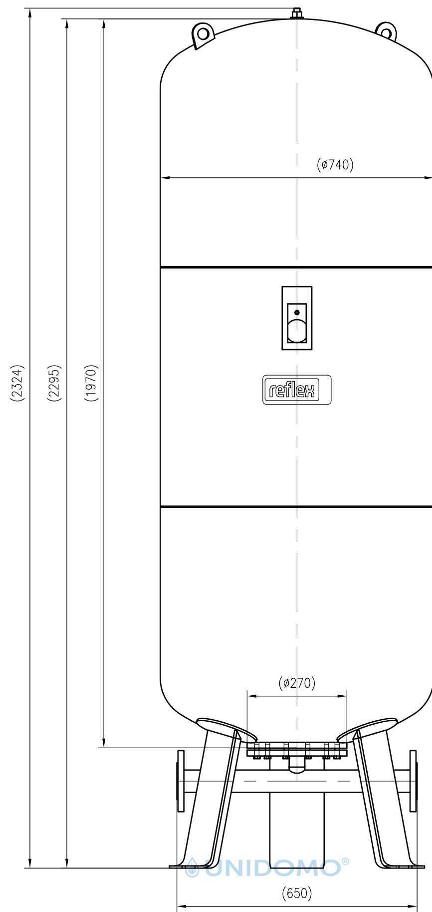
Front view
