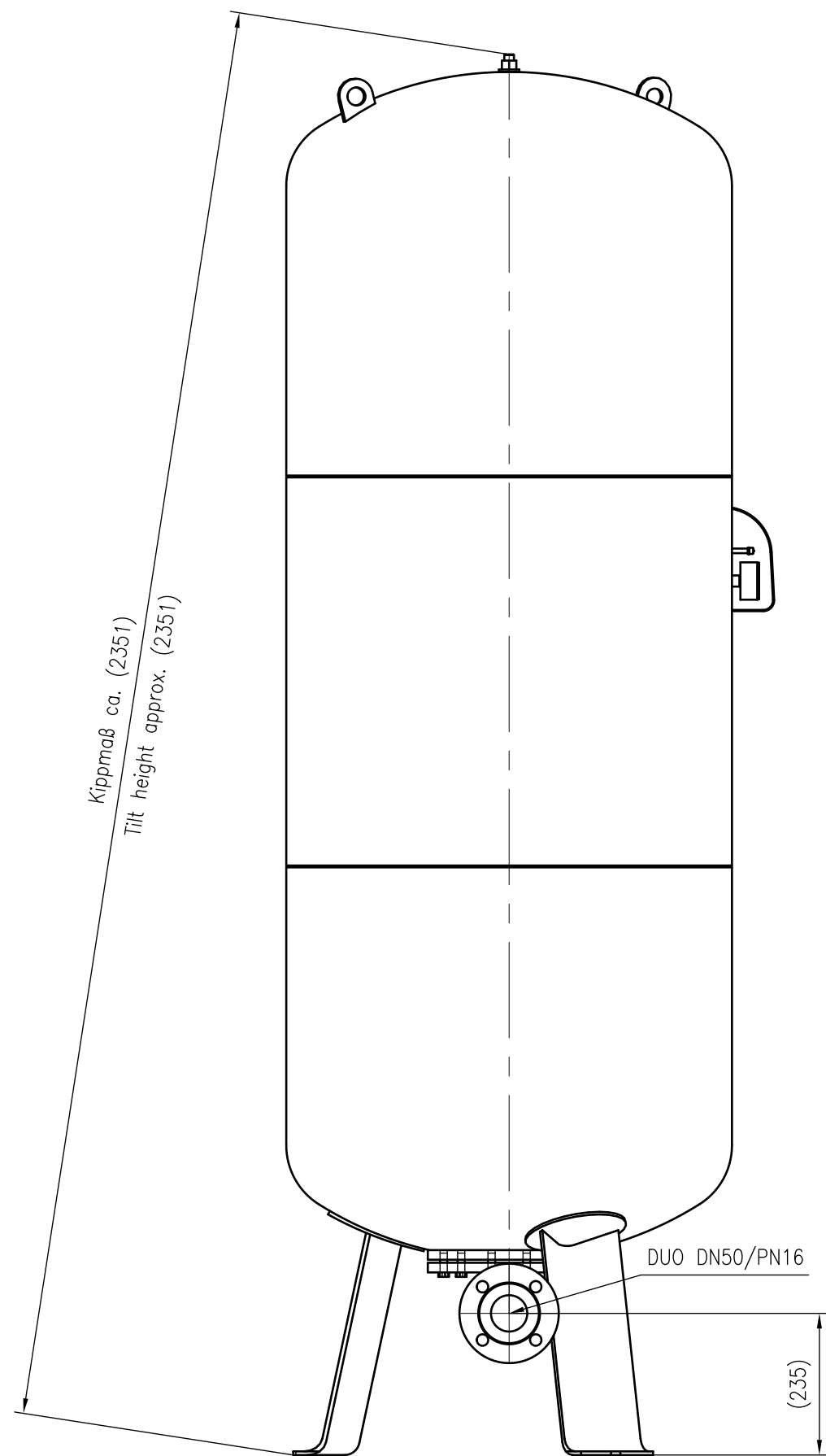
Side view
