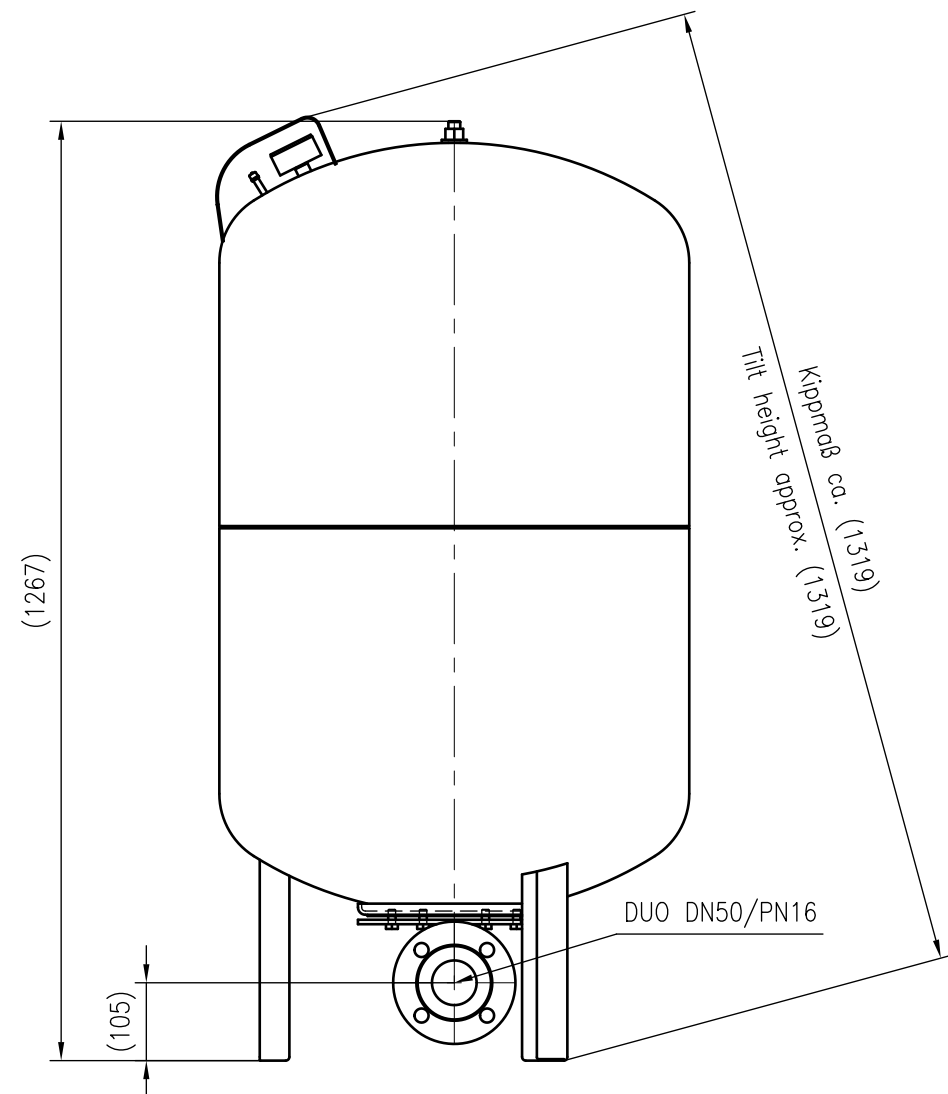
Side view
