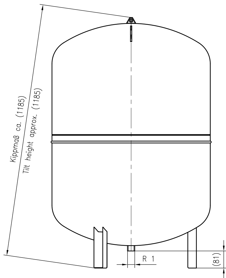
Side view
