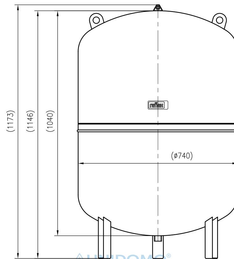
Front view
