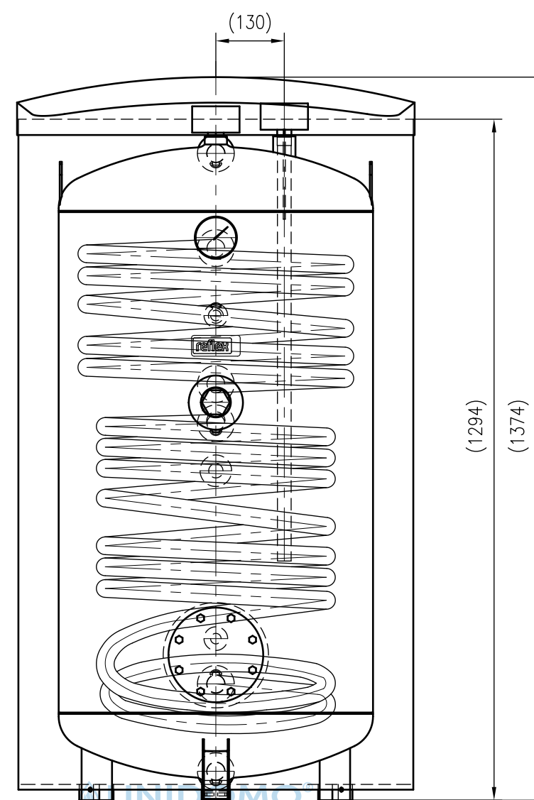
Front view
