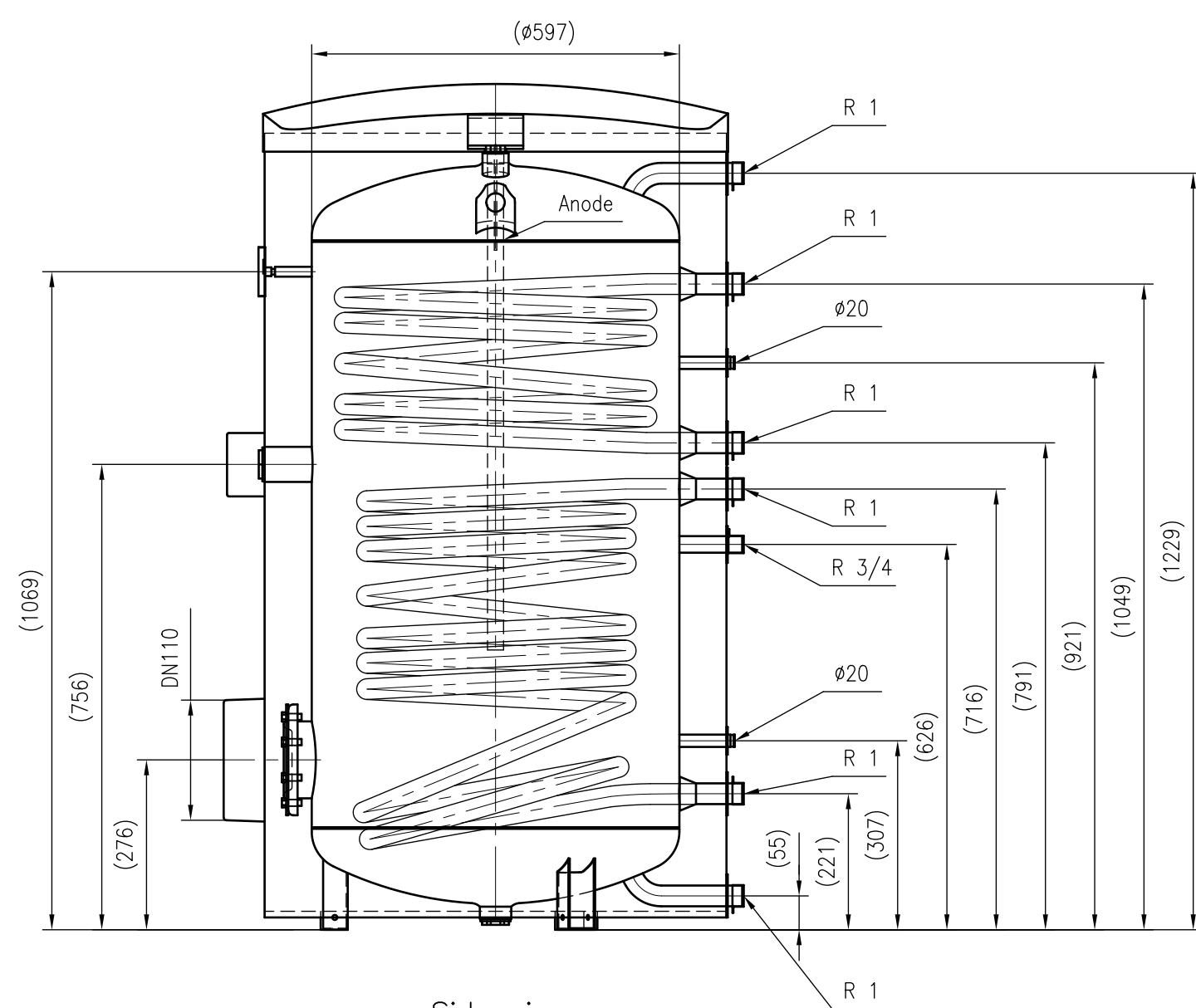
Side view
