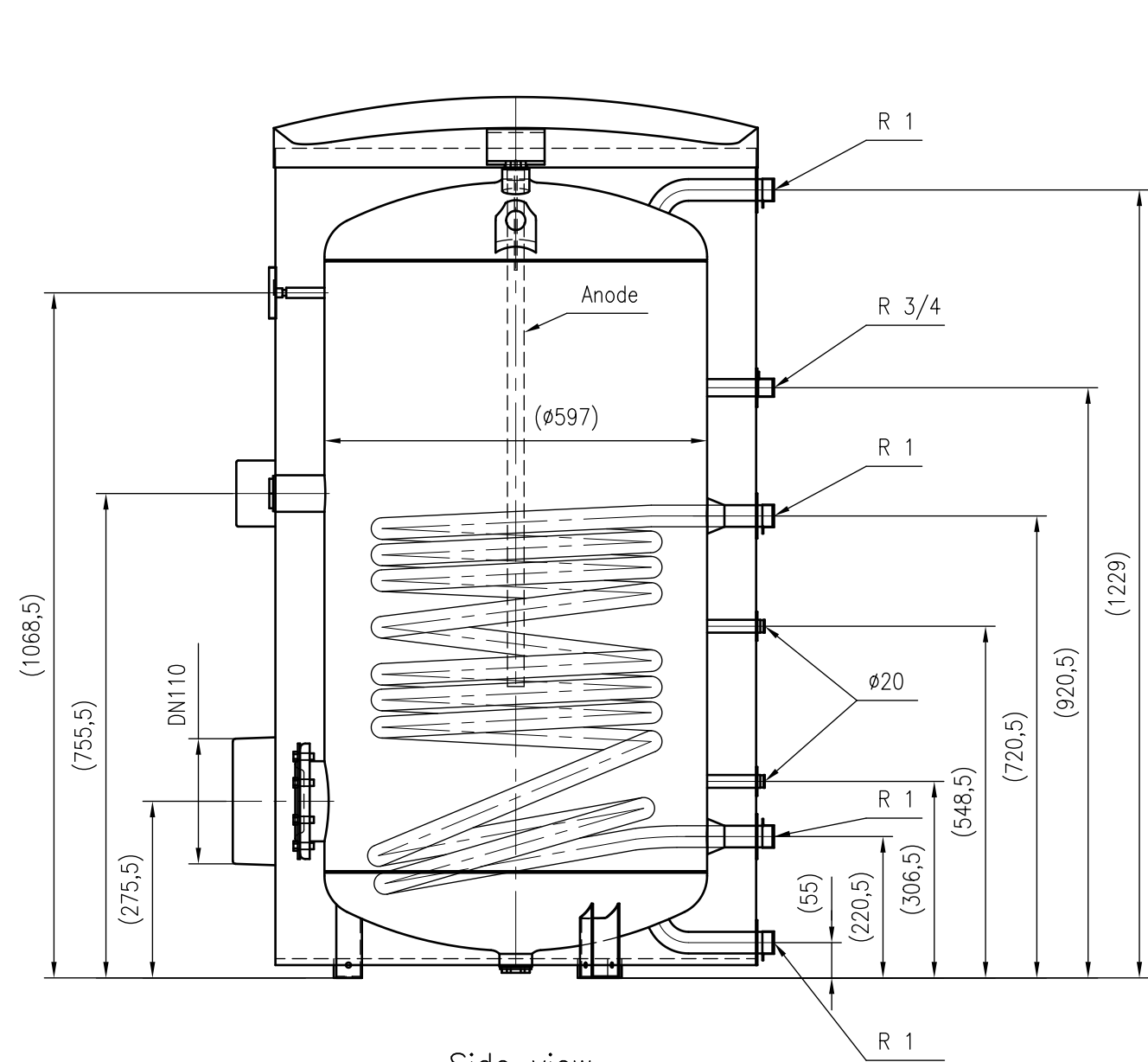
Side view
