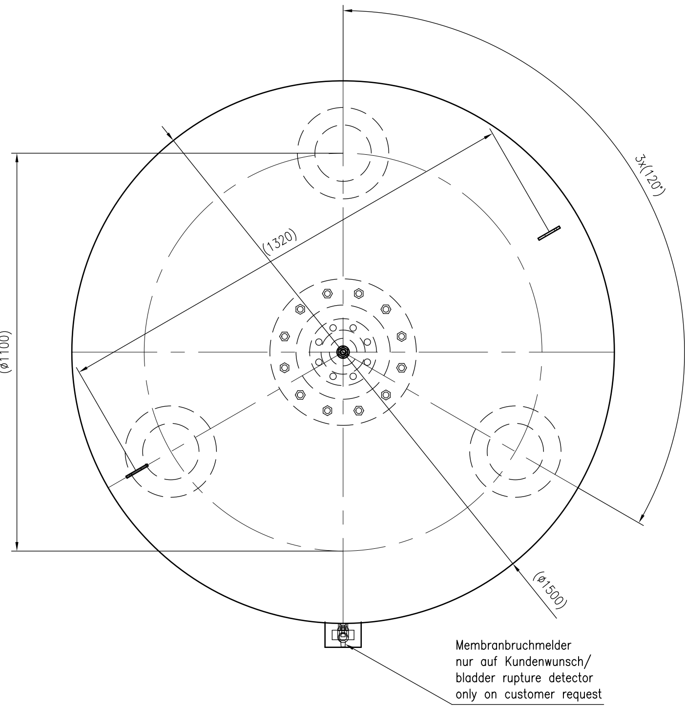
Top view
