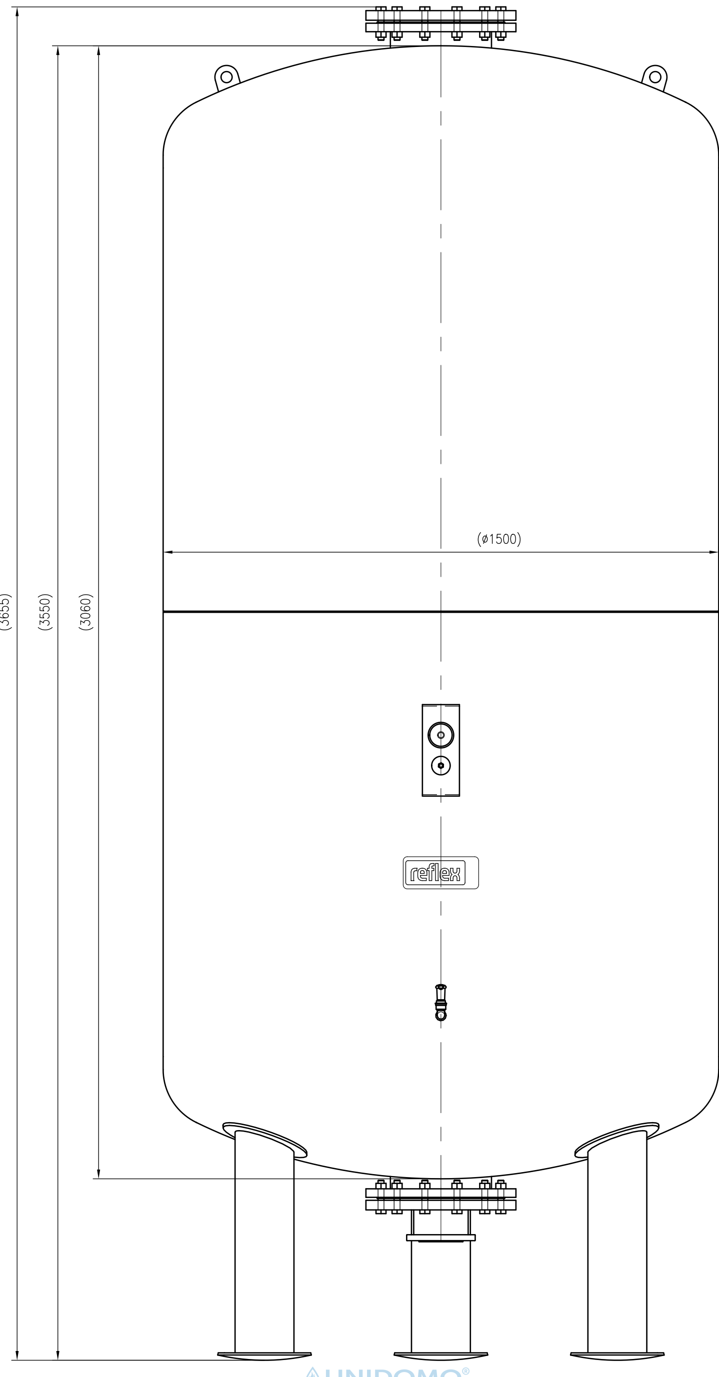
Front view
