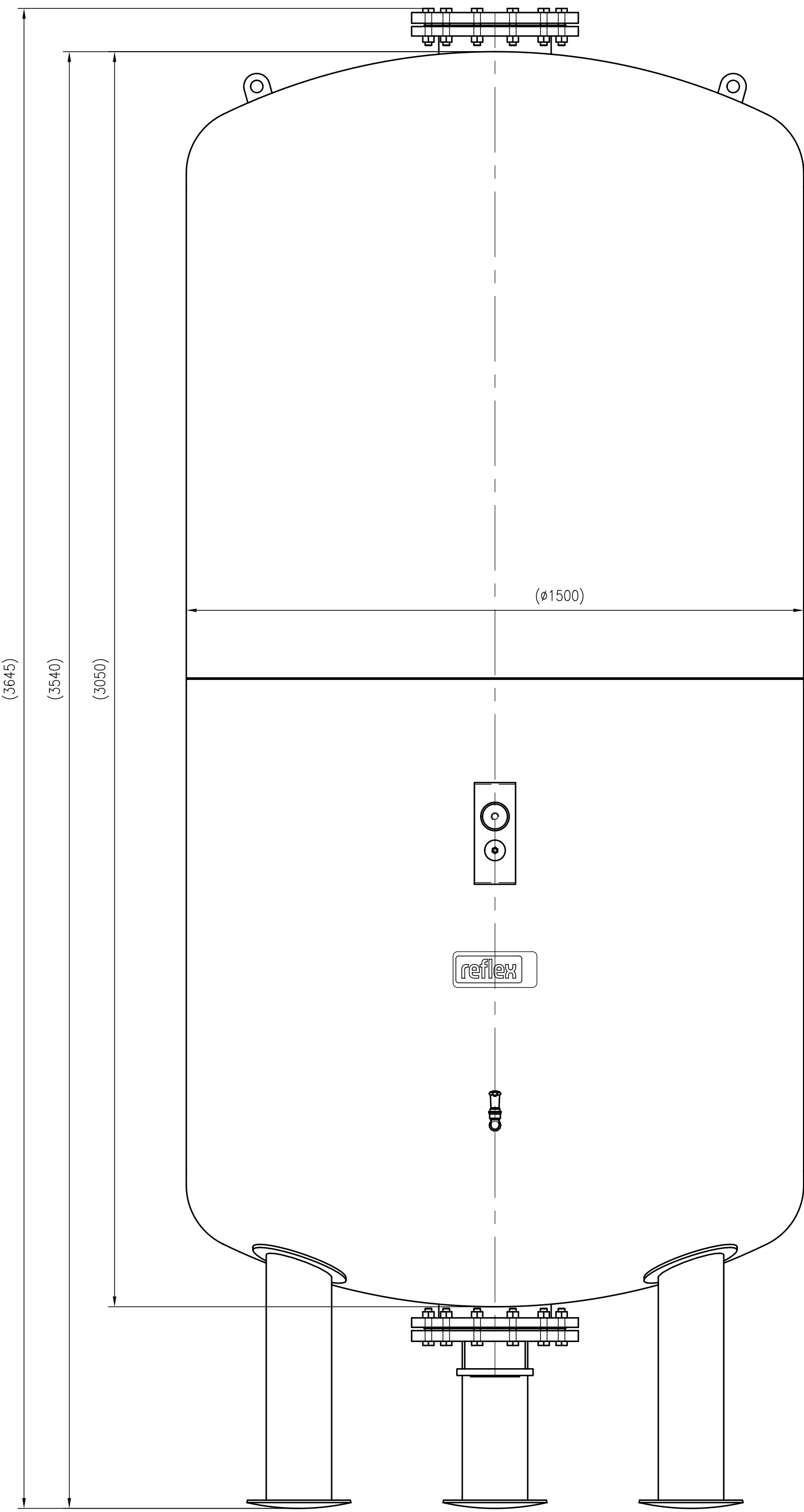
Front view
