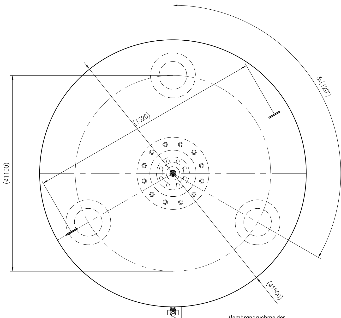
Top view
