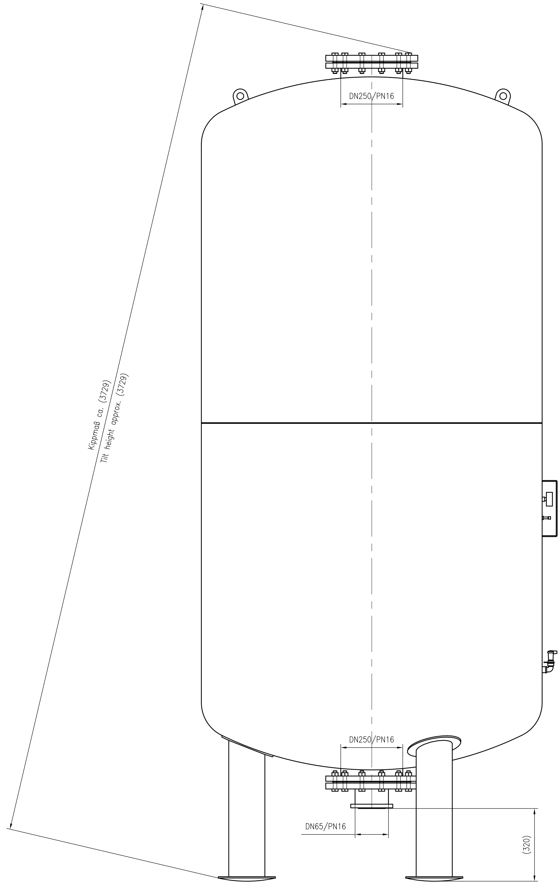
Side view
