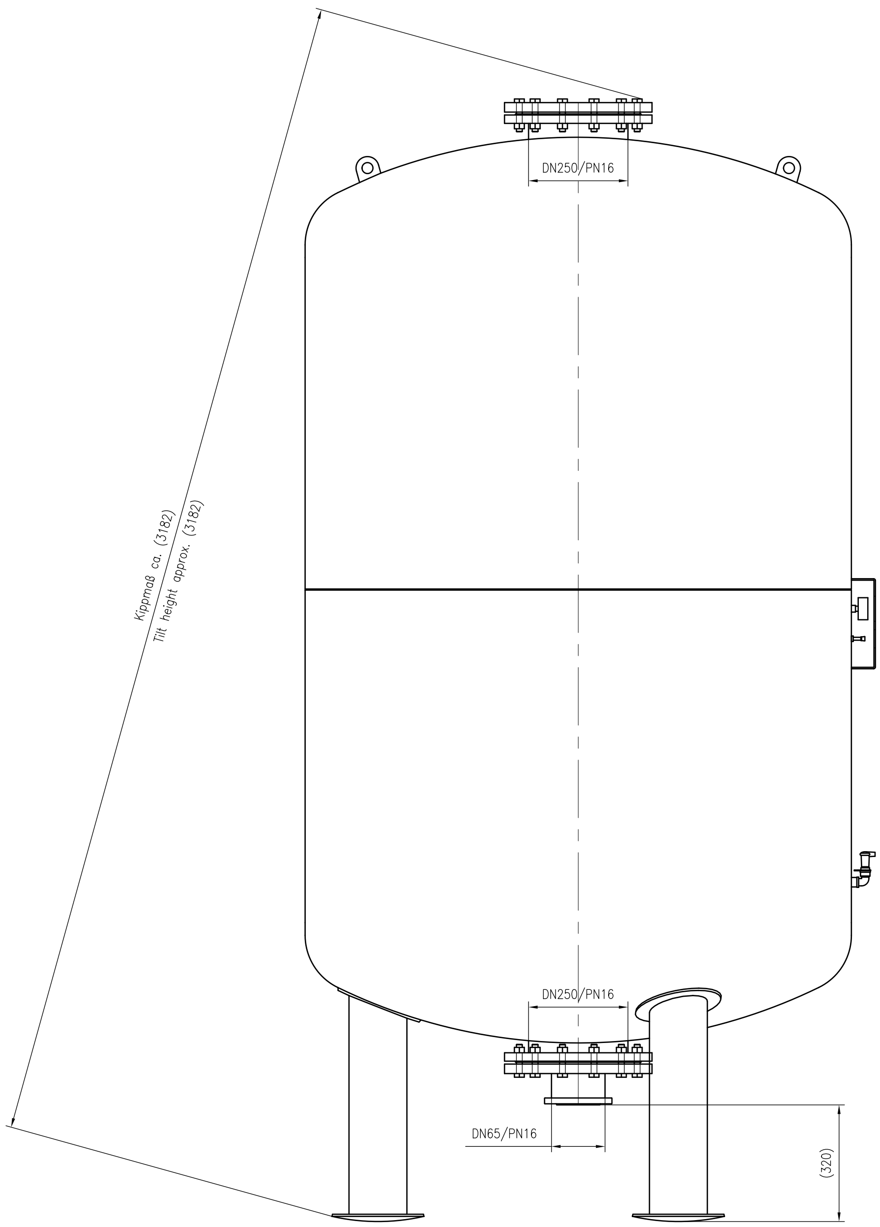
Side view
