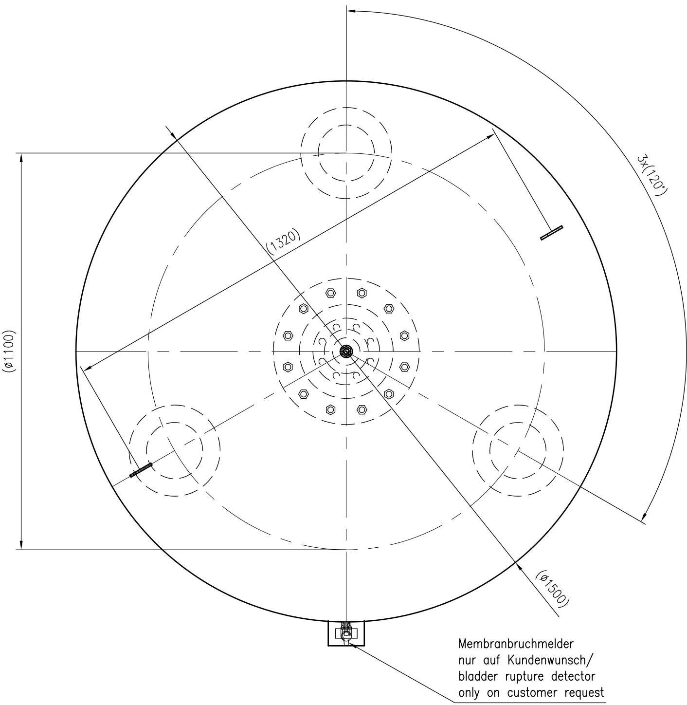
Top view
