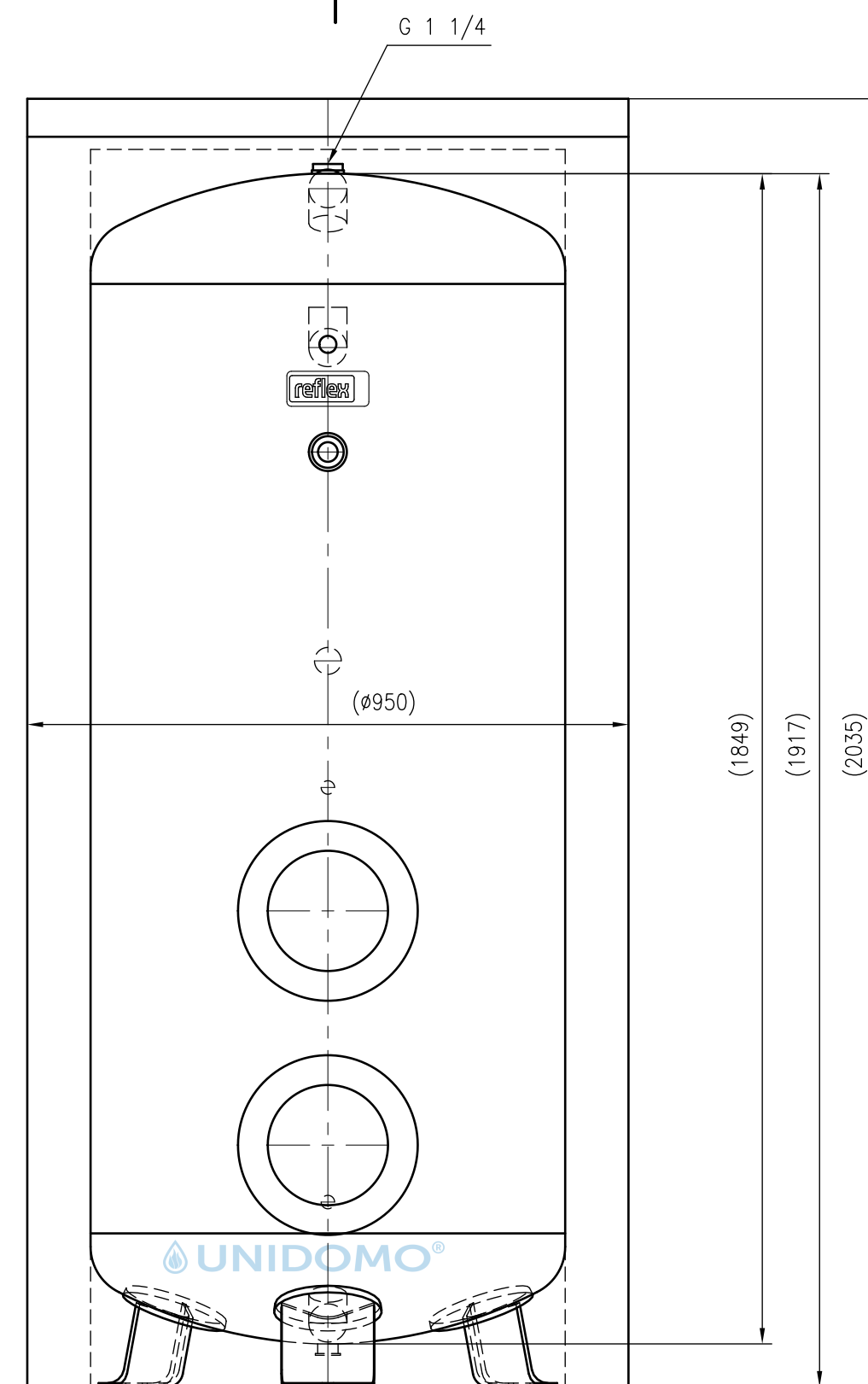
Front view
