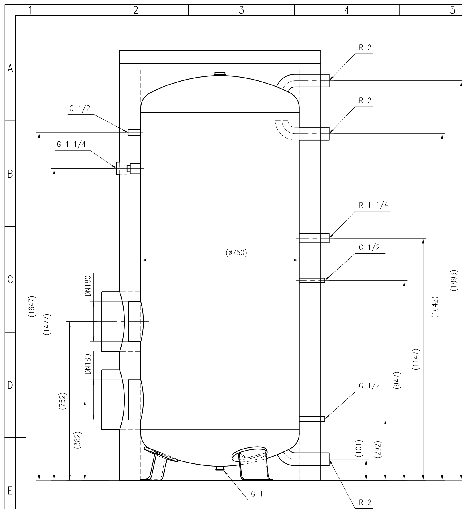
Side view
