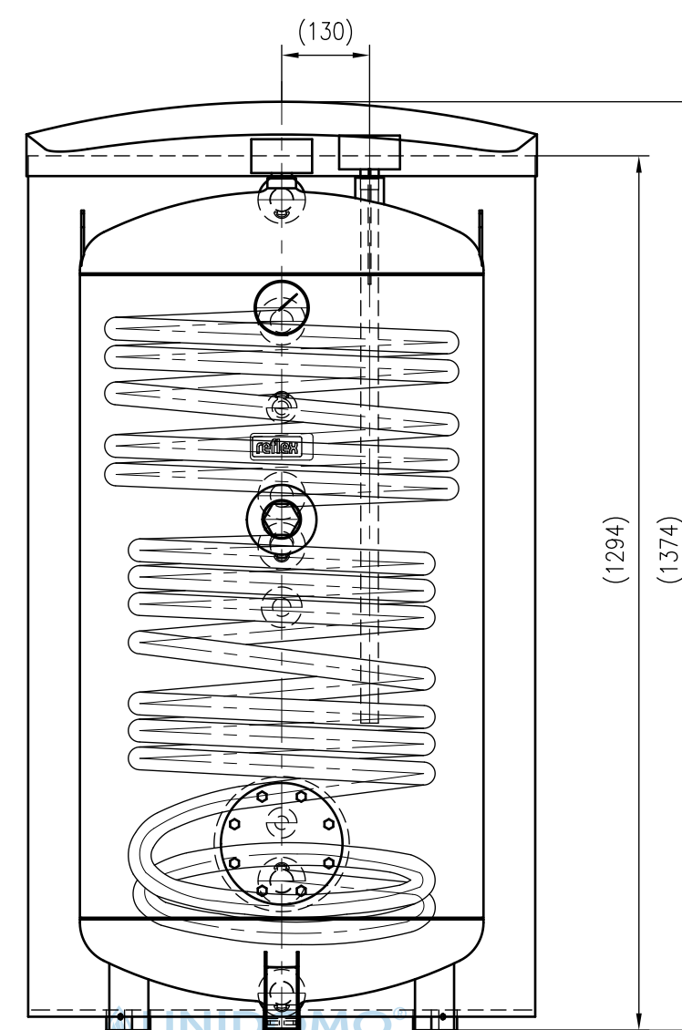
Front view
