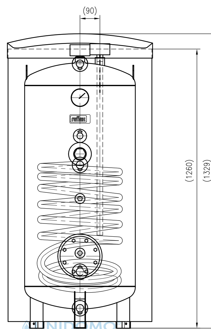
Front view
