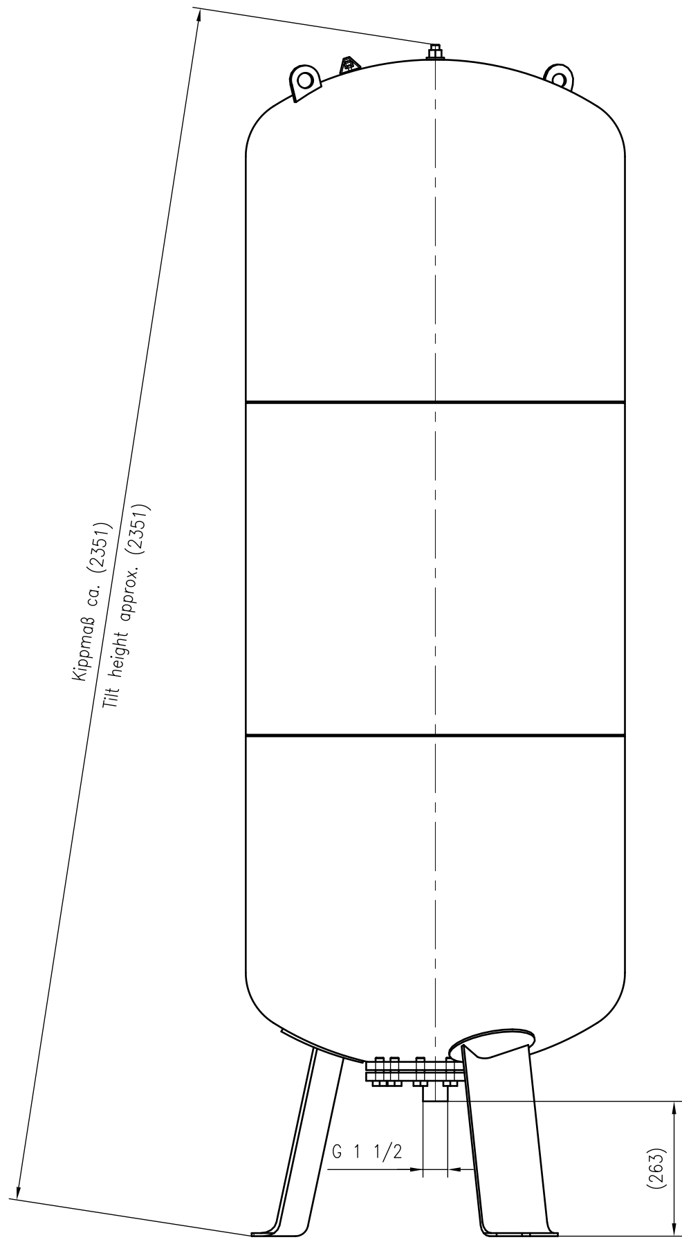
Side view
