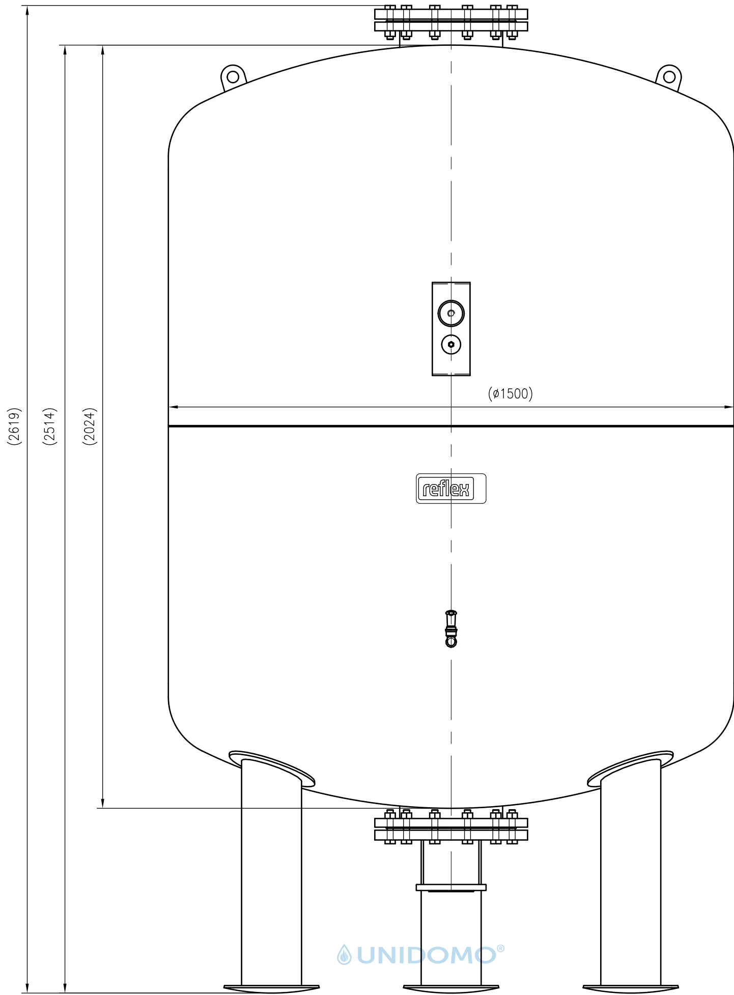
Front view
