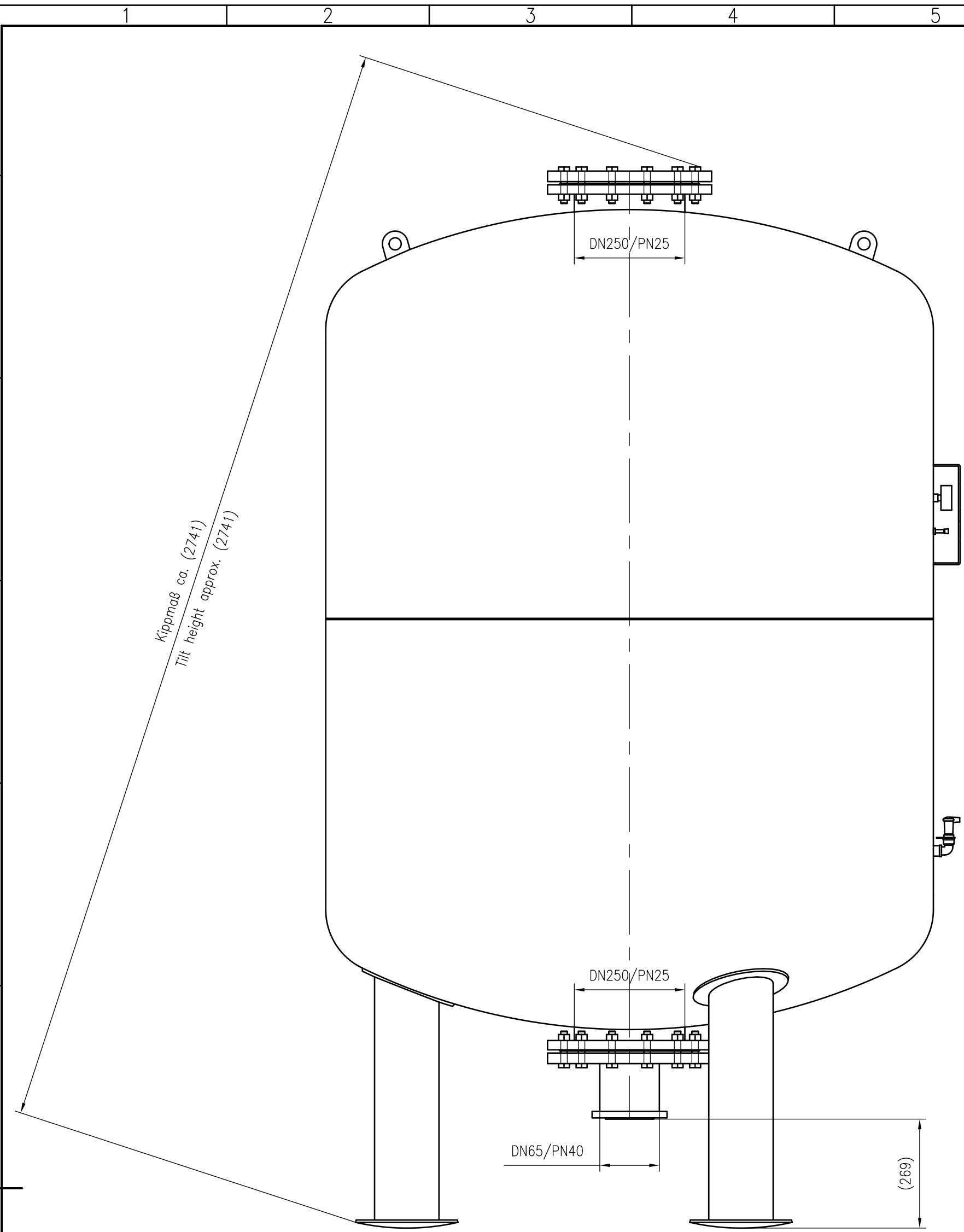
Side view
