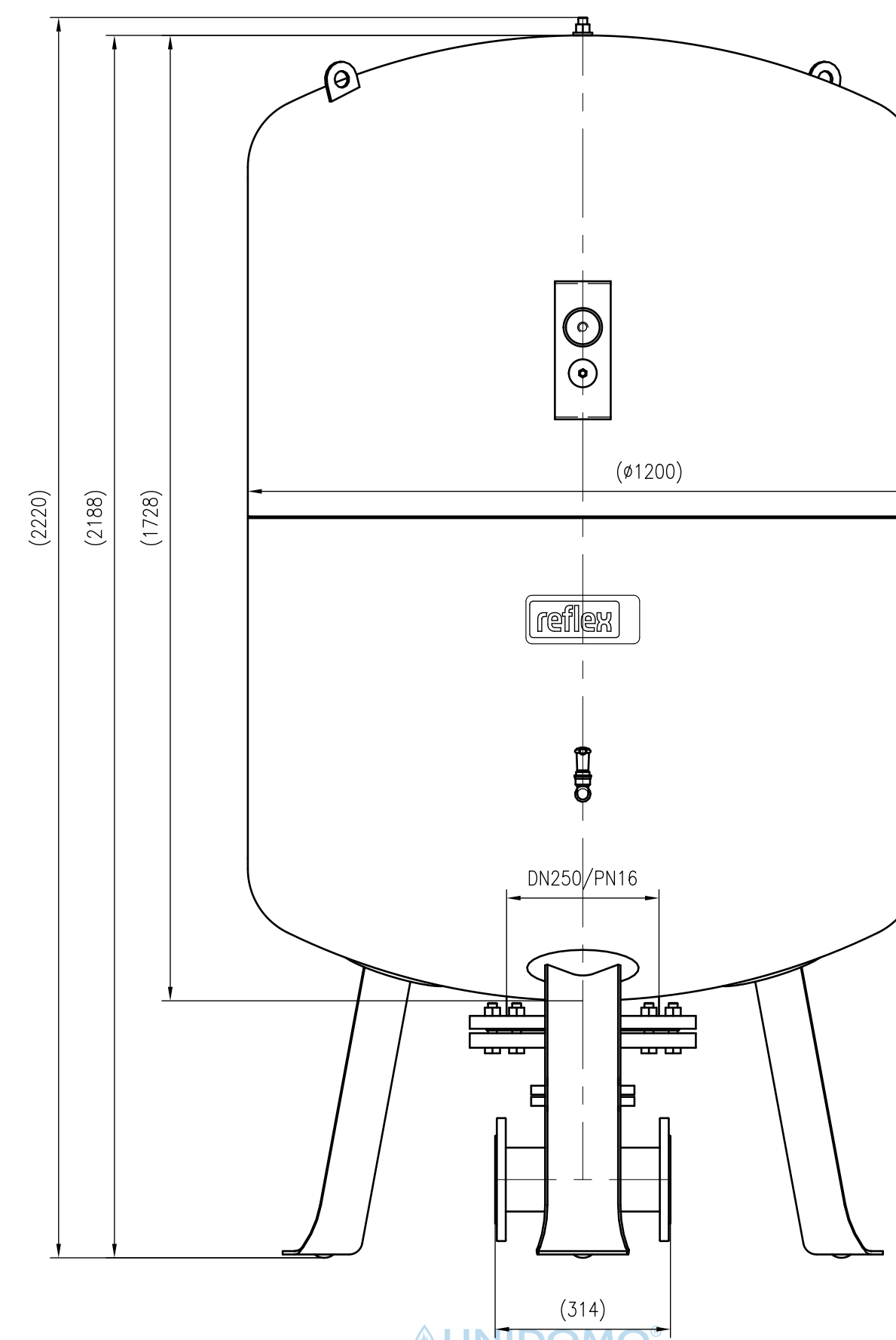
Front view
