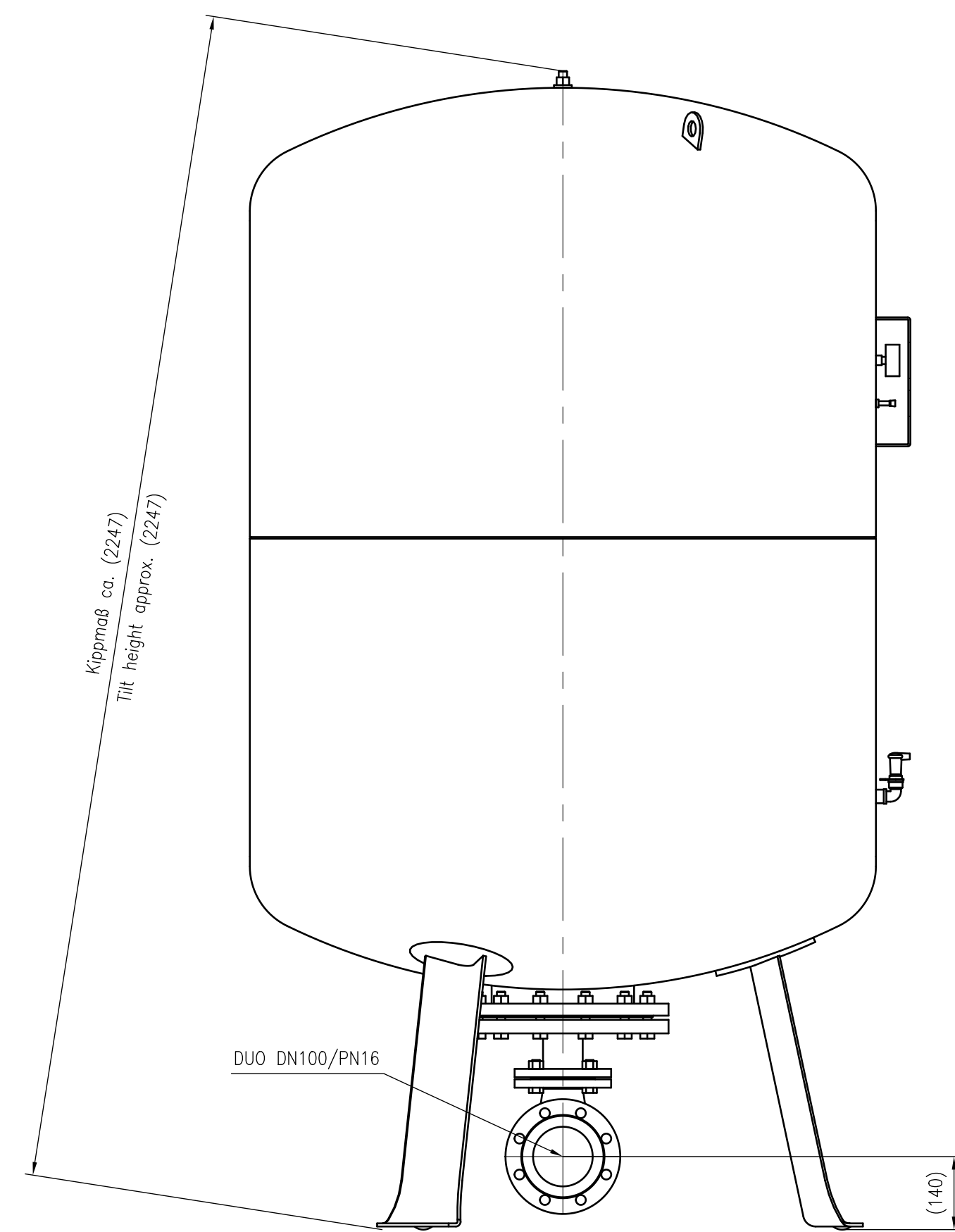
Side view
