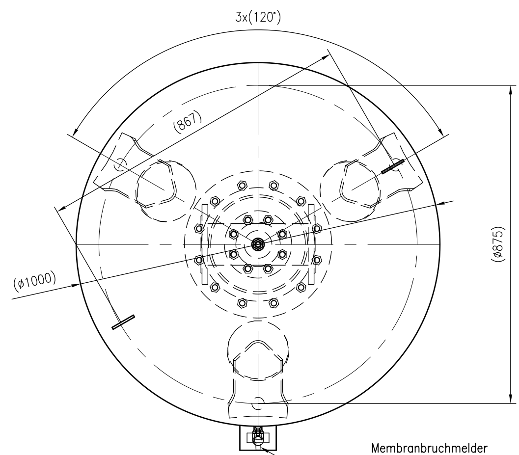
Top view
