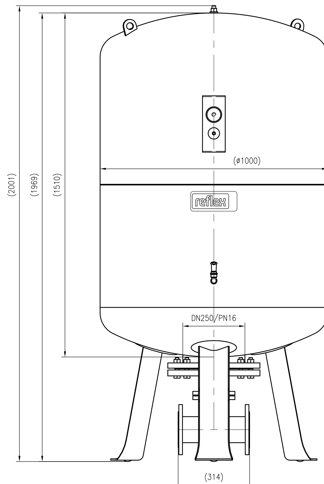
Front view
