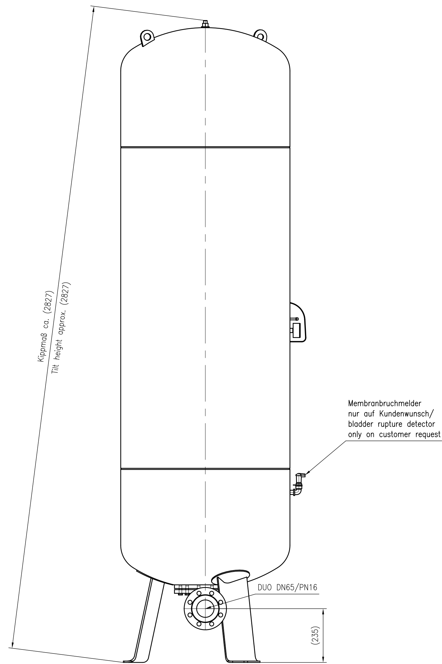
Side view
