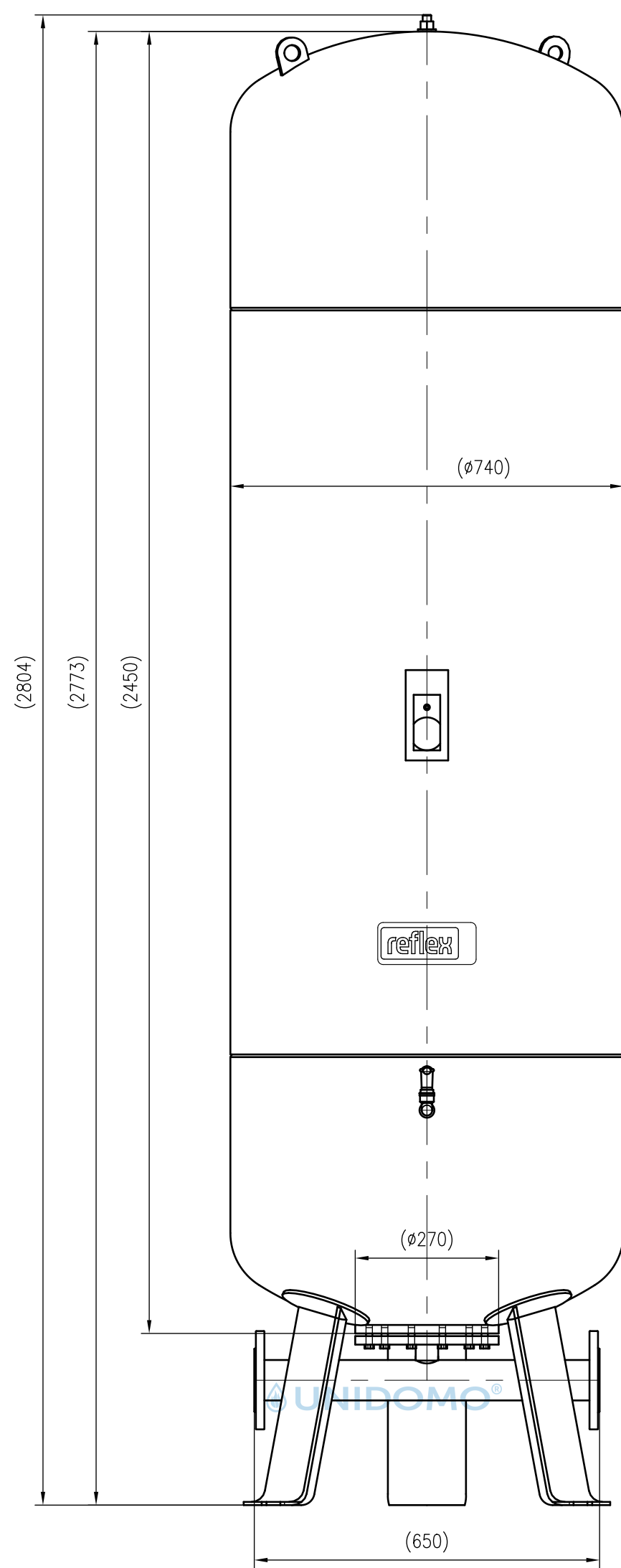
Front view
