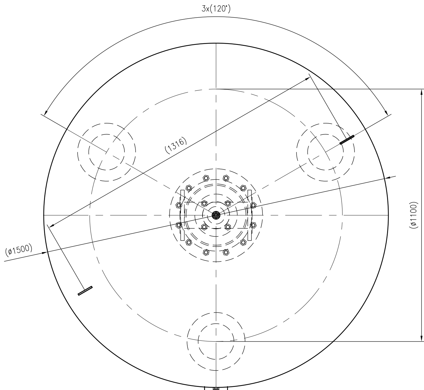
Top view
