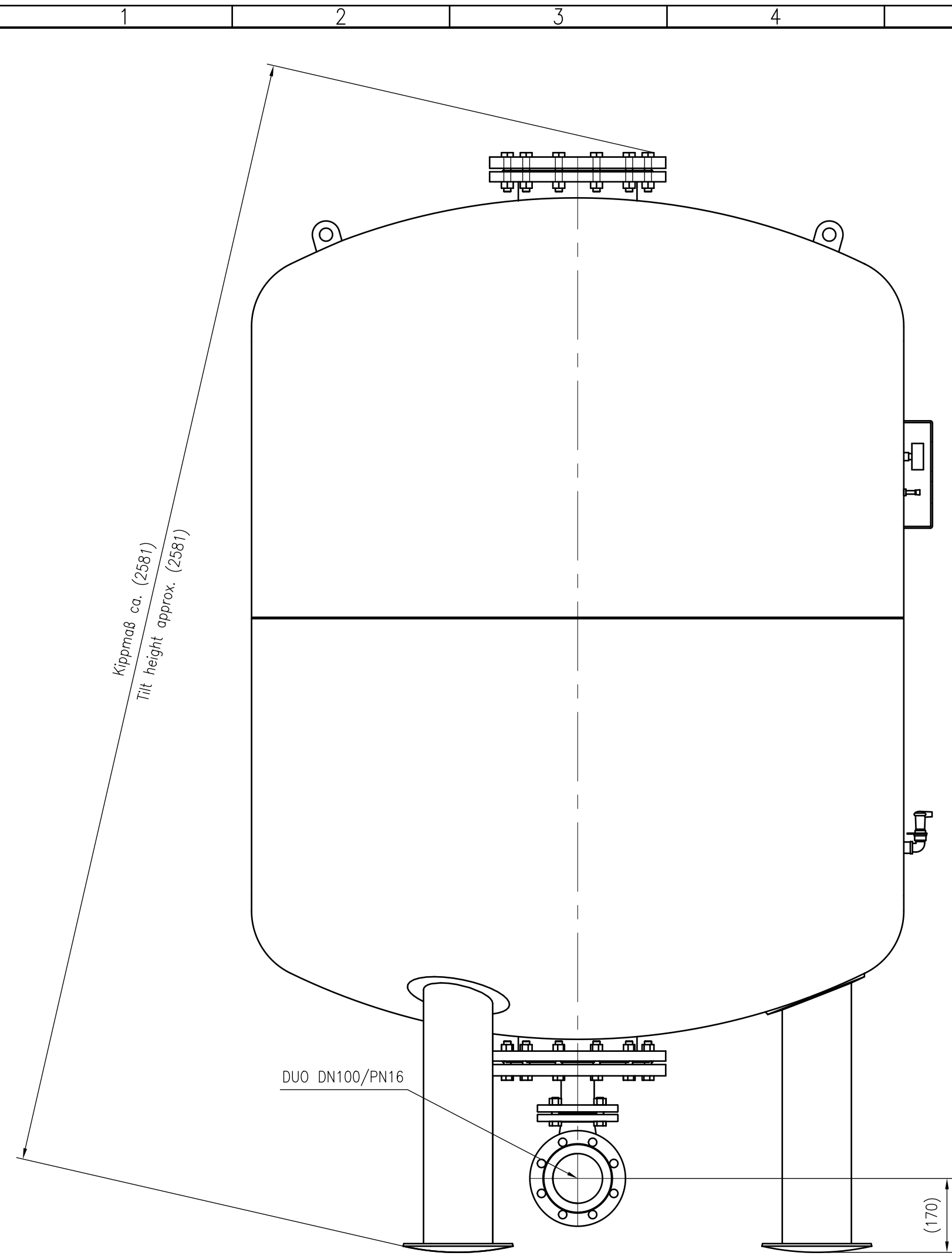
Side view
