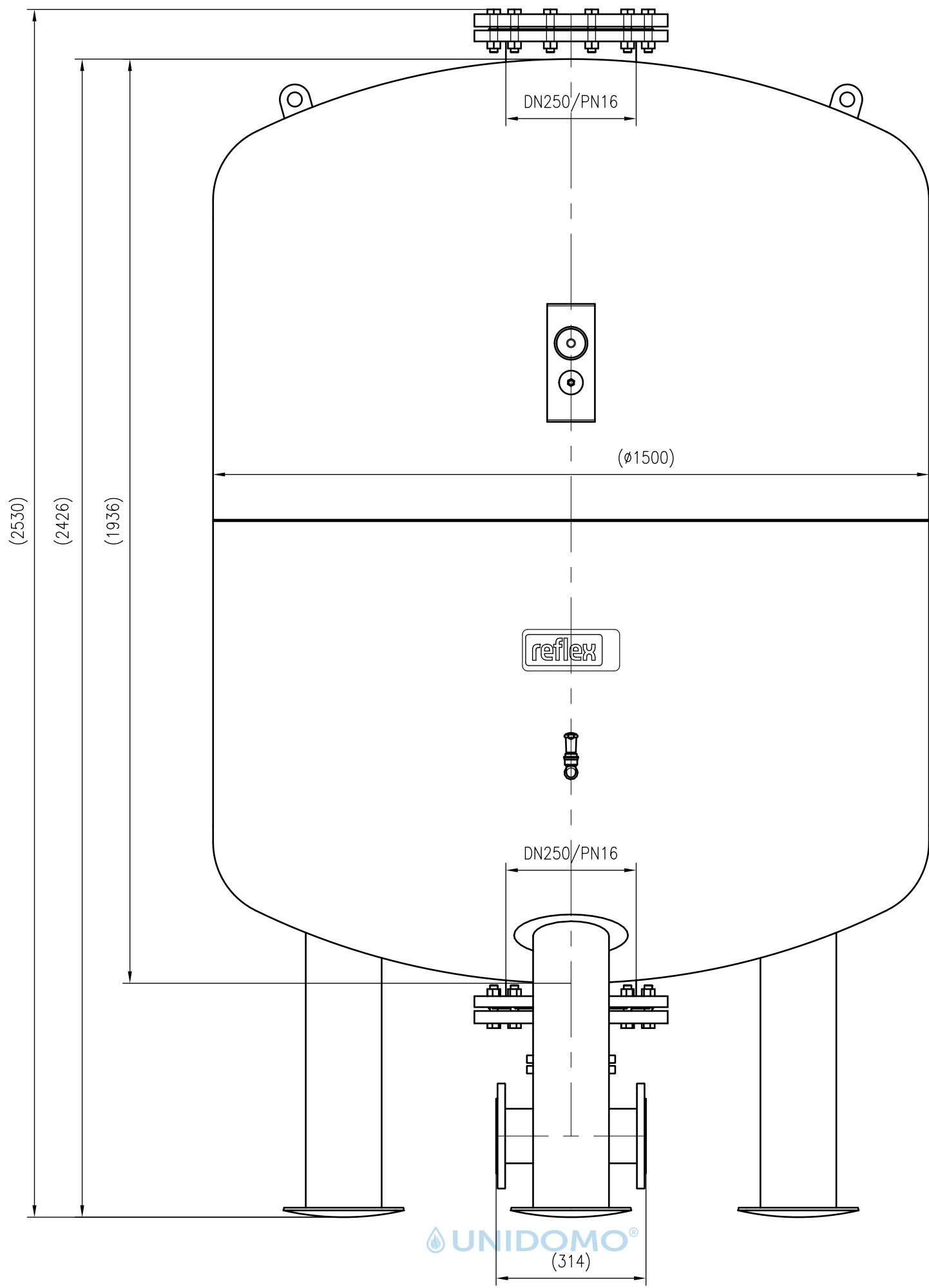
Front view
