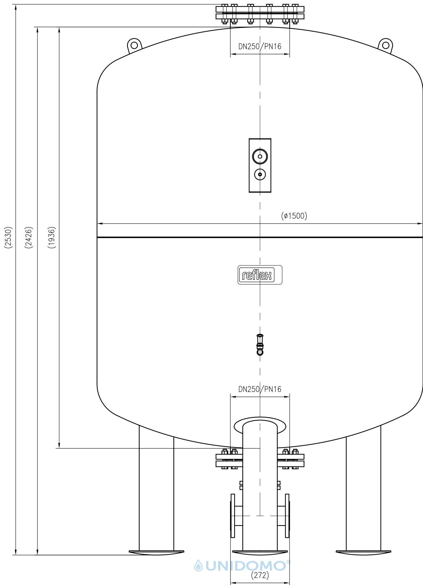
Front view
