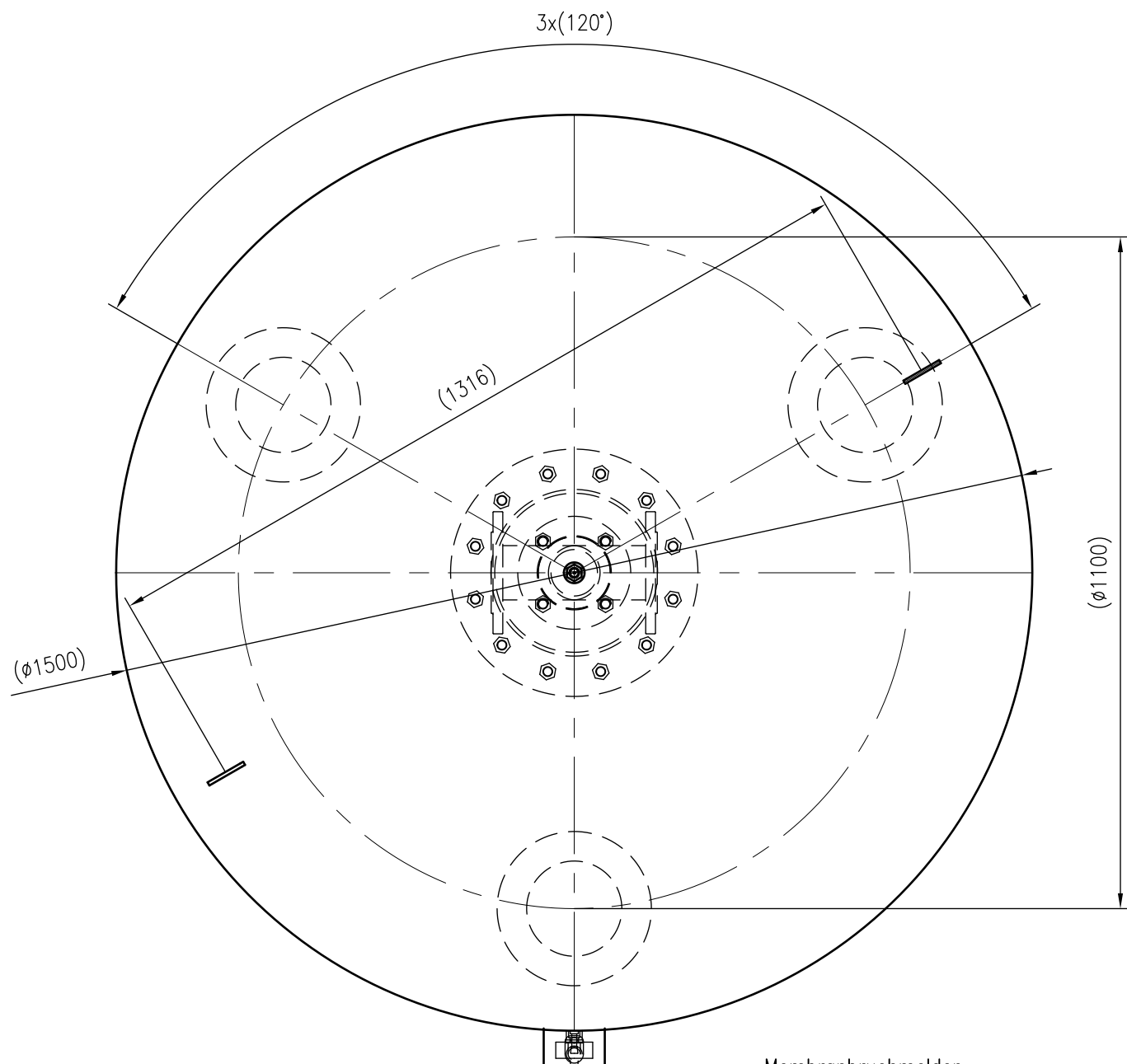
Top view
