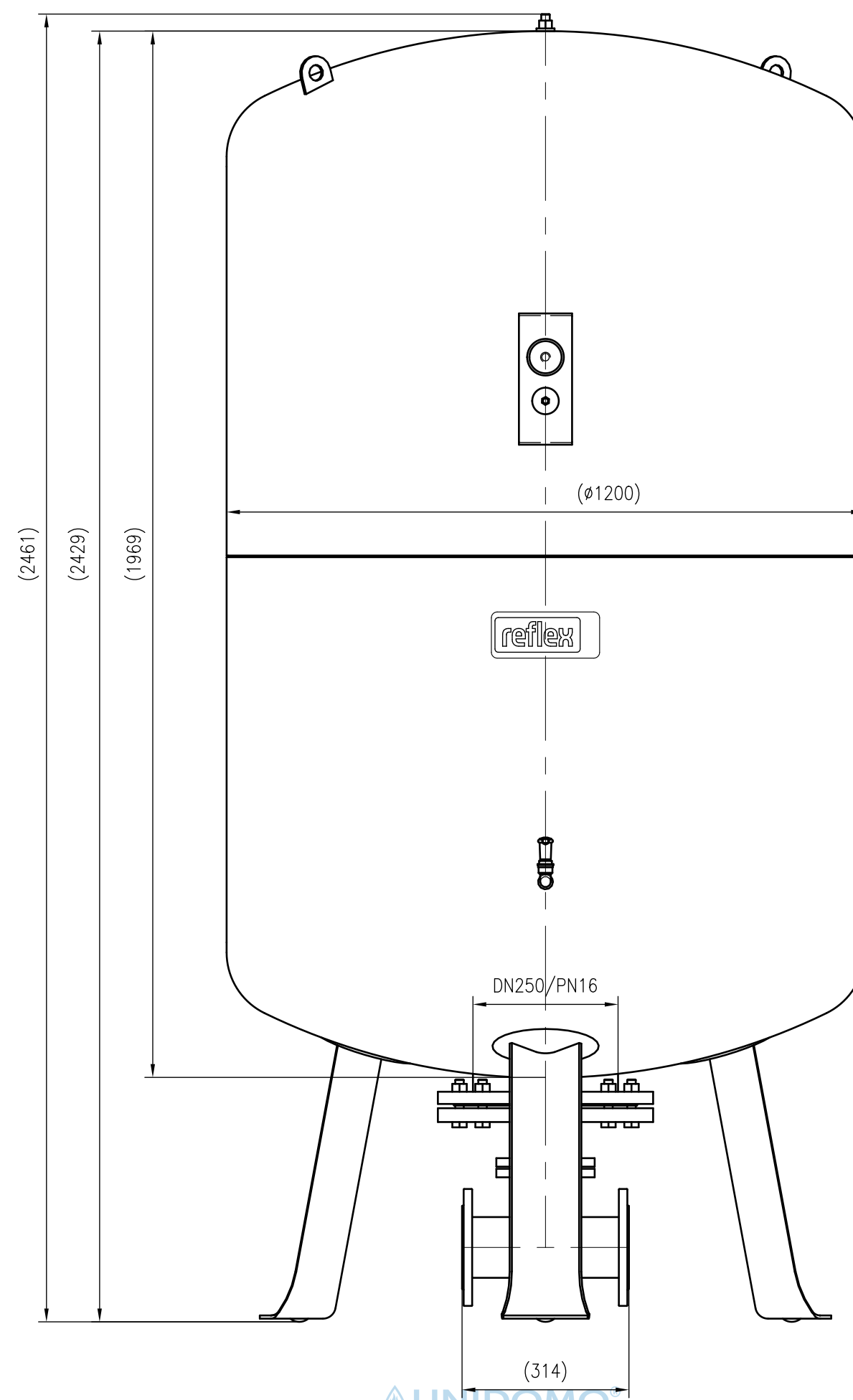
Front view
