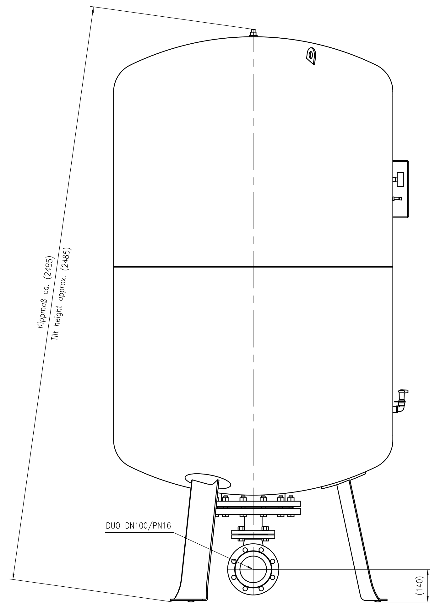
Side view
