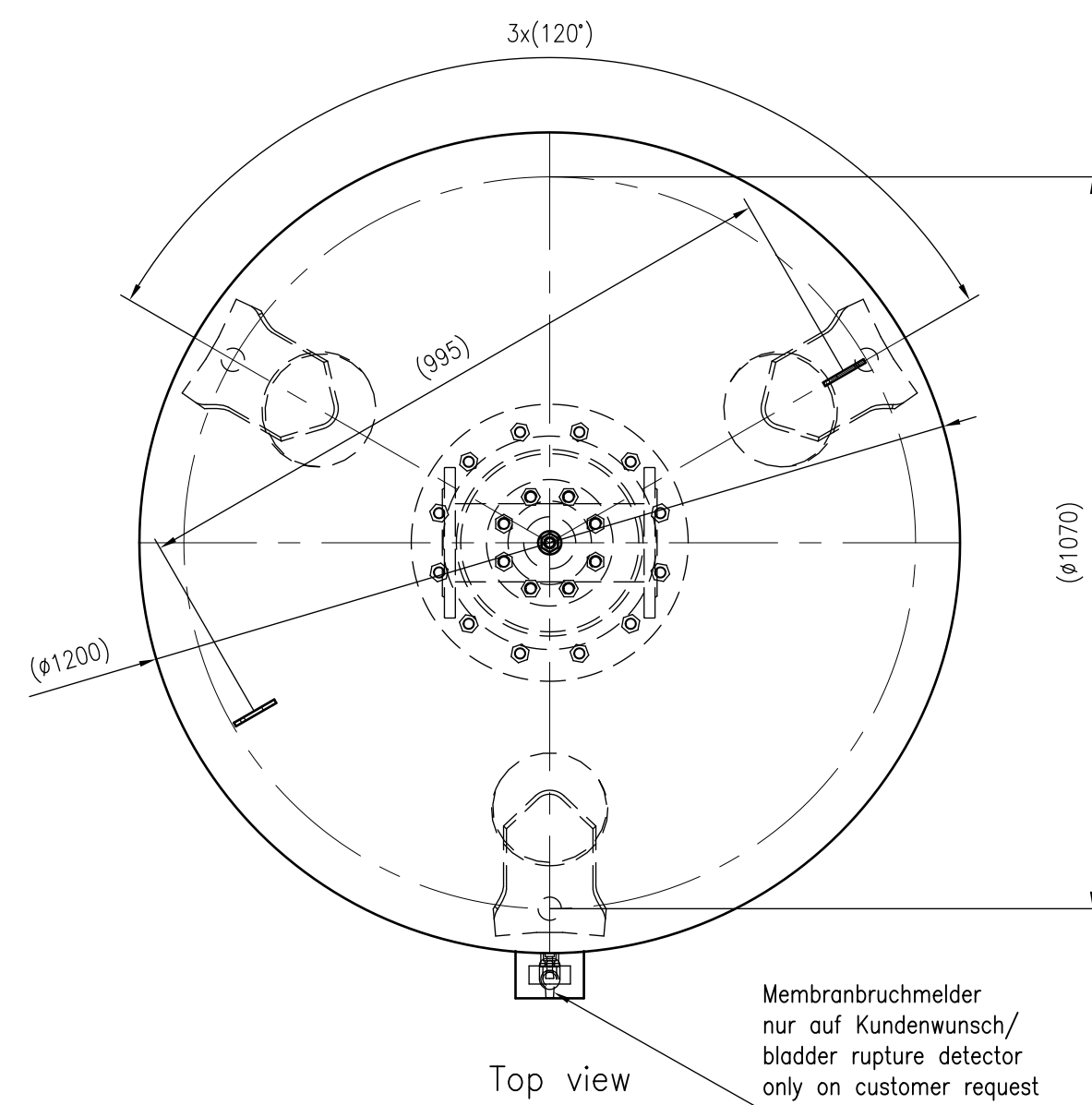
Top view
