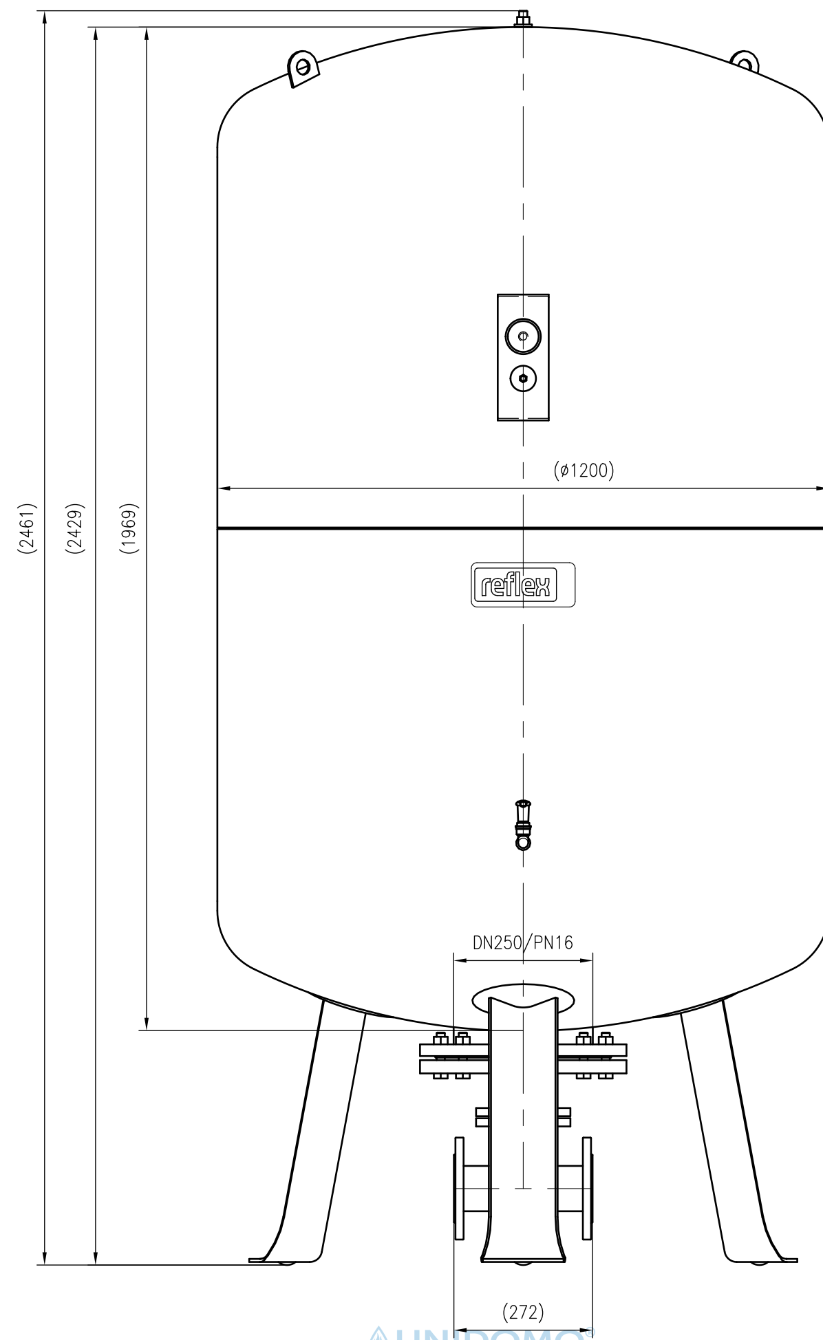
Front view
