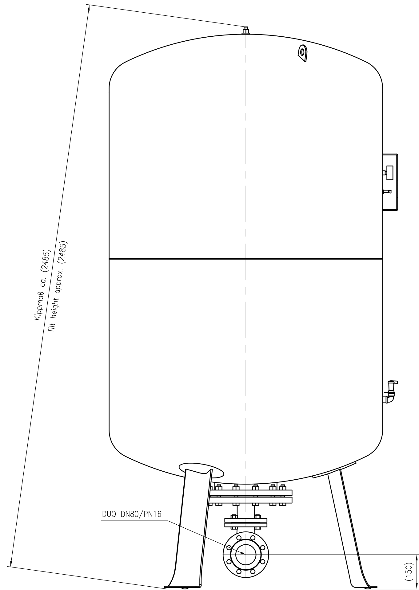
Side view
