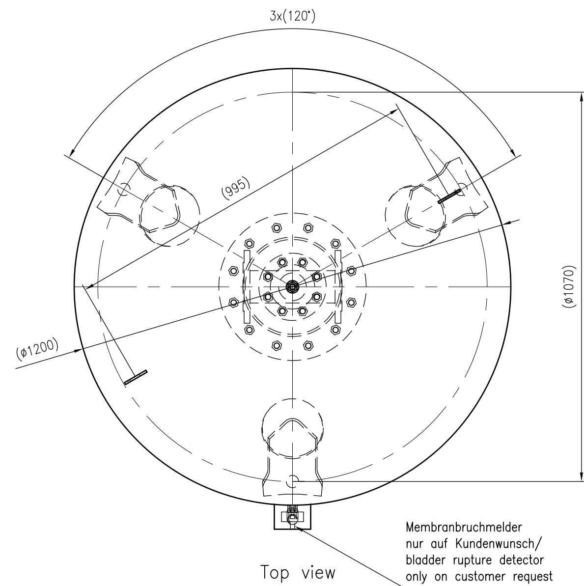
Top view
