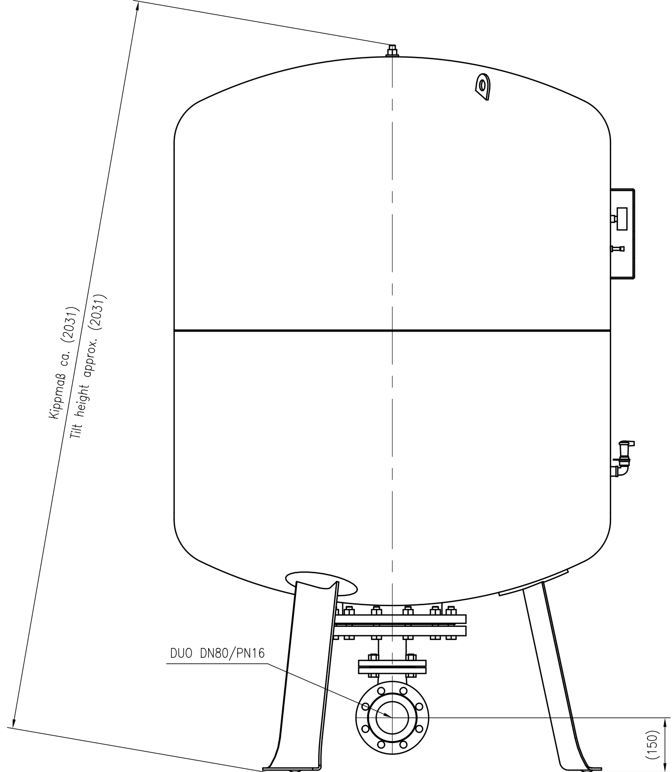
Side view
