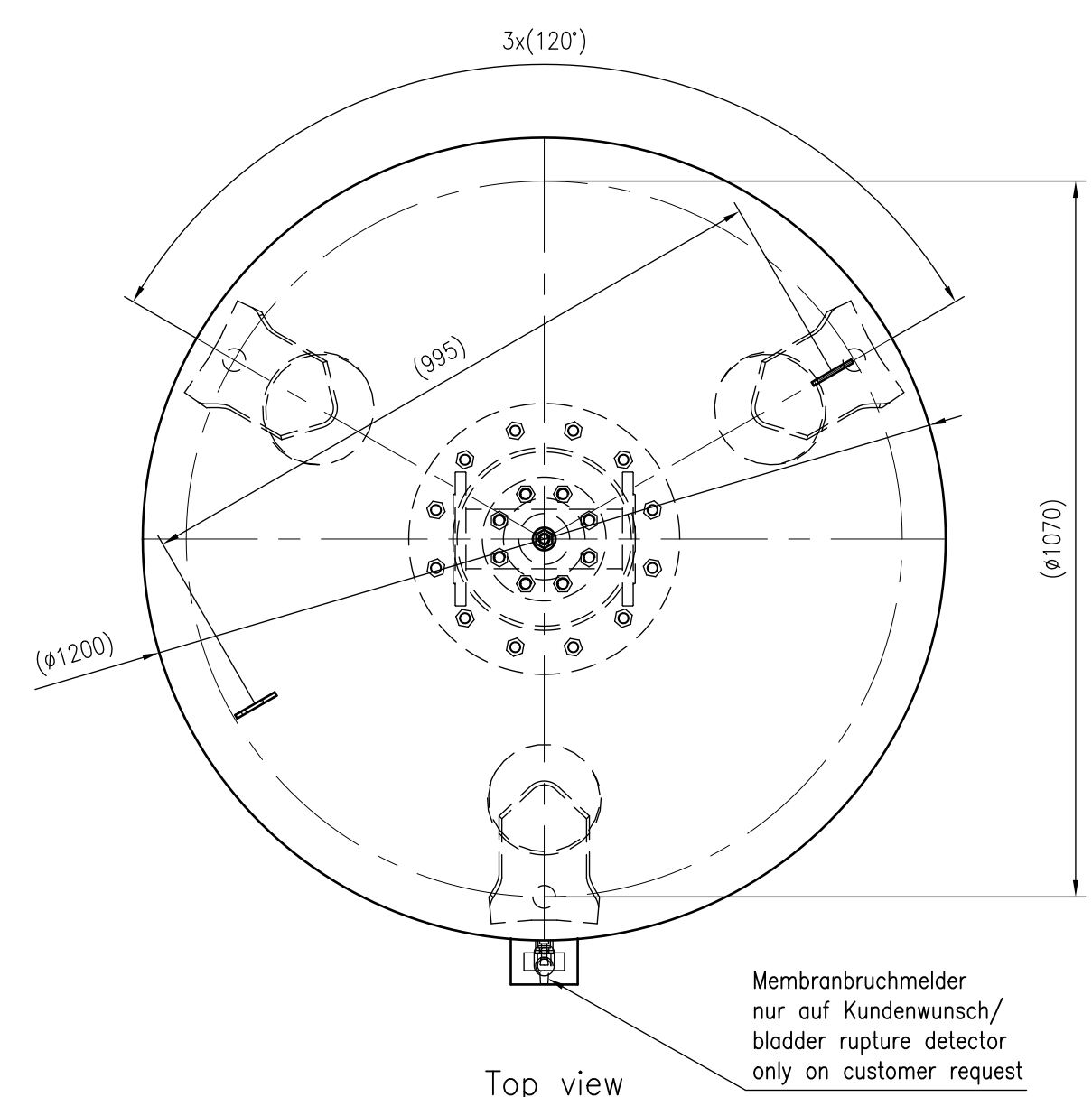
Top view
