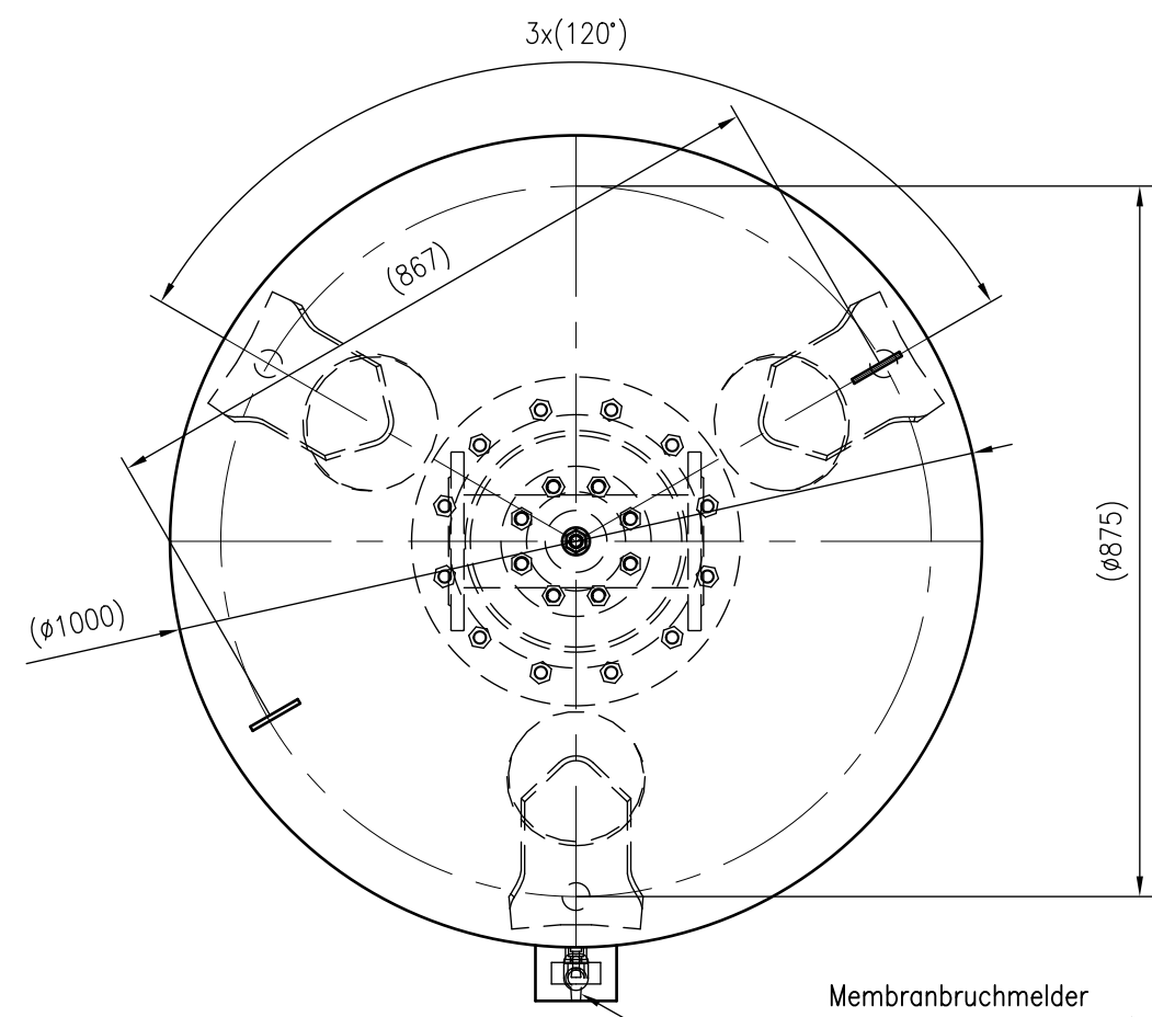
Top view
