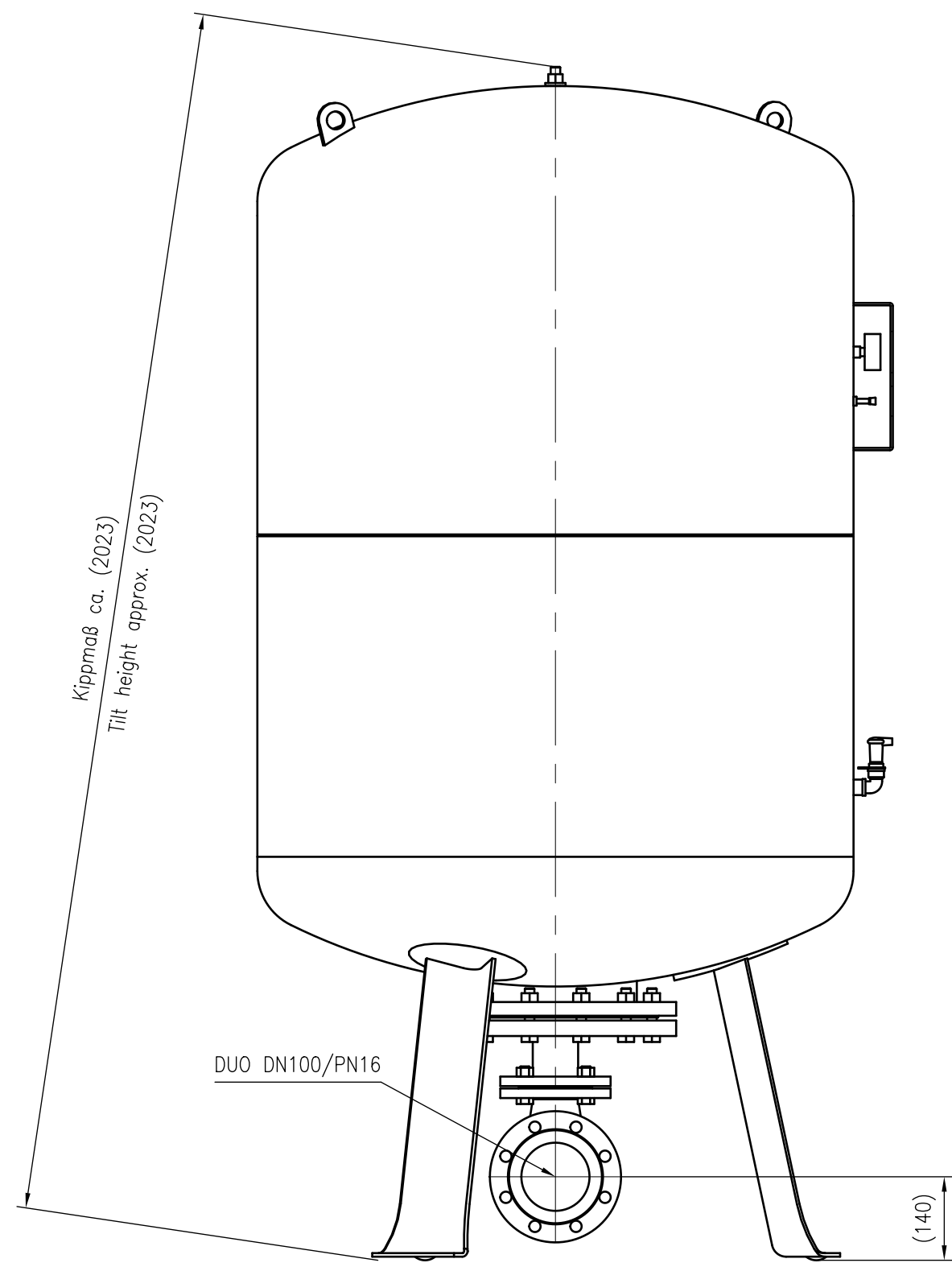
Side view
