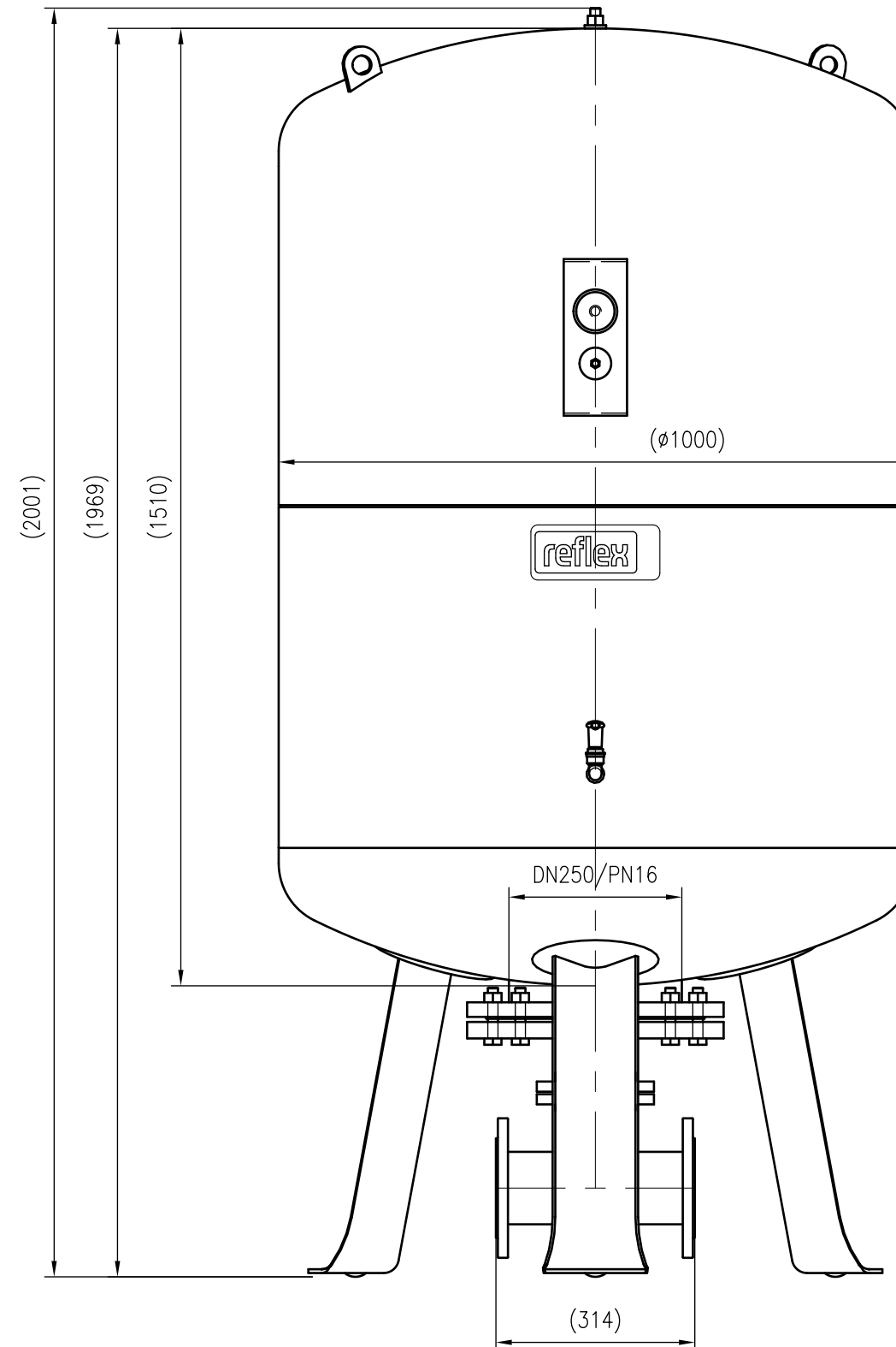
Front view
