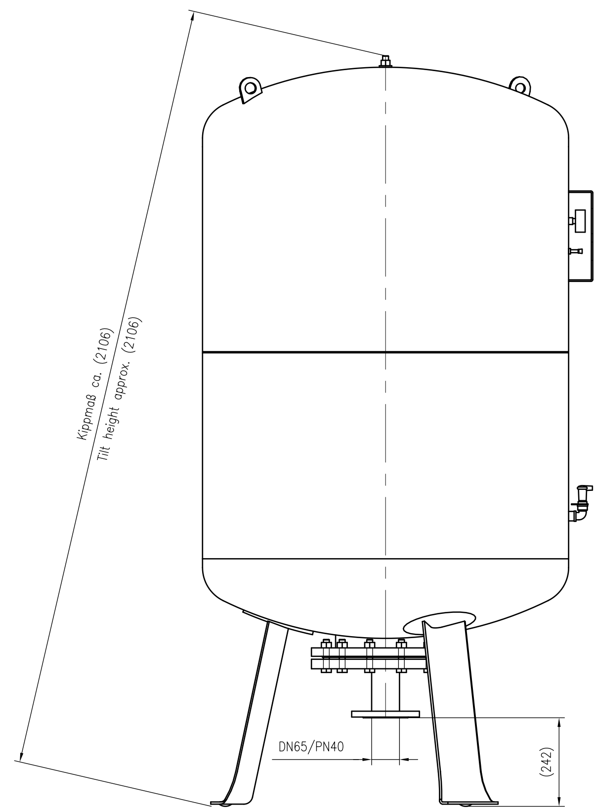
Side view
