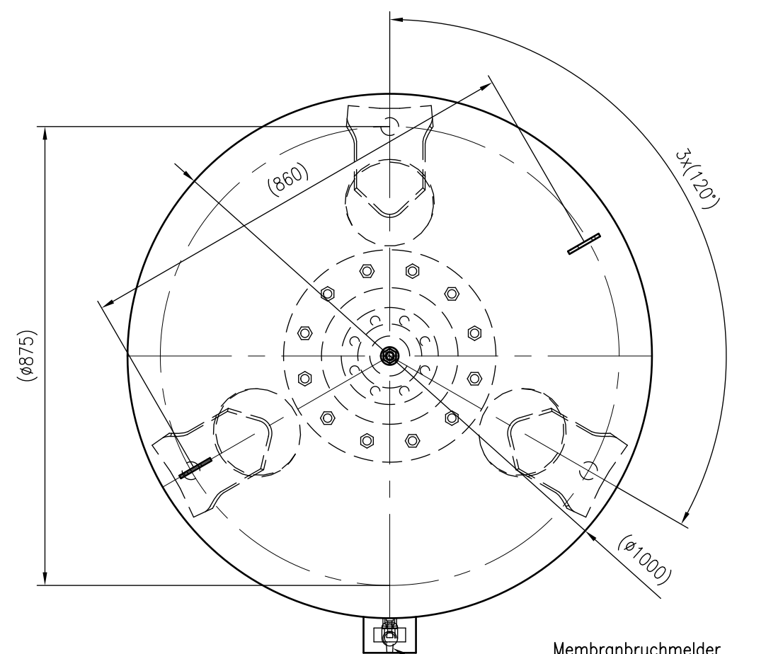
Top view
