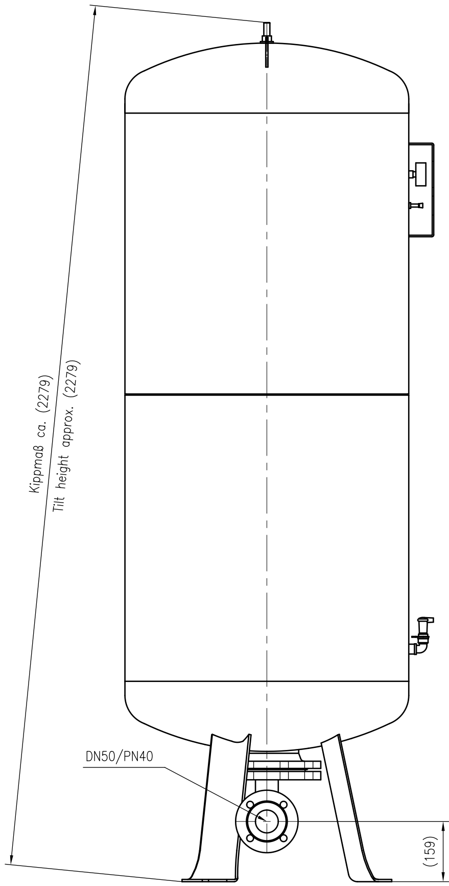
Side view
