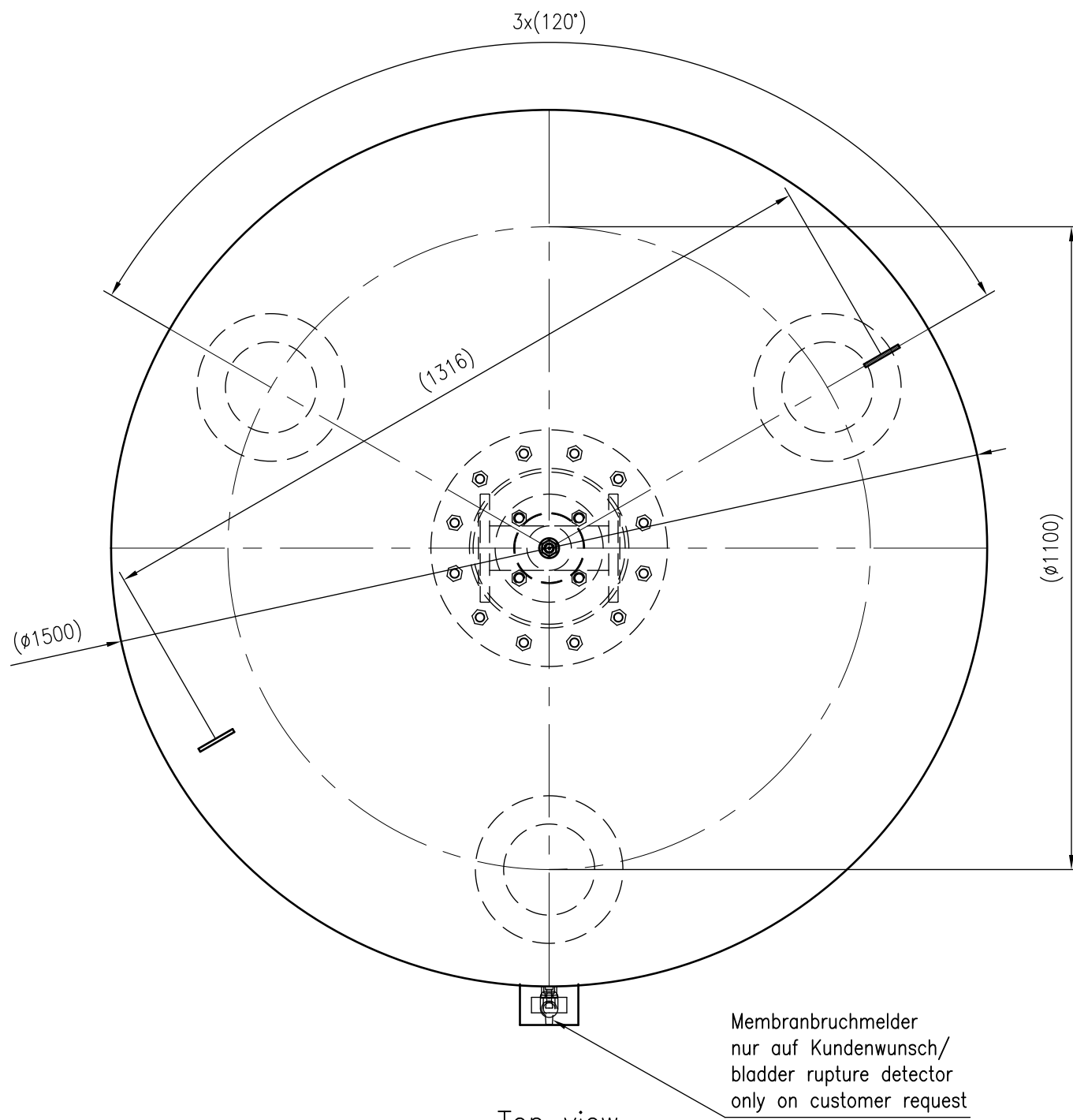
Top view
