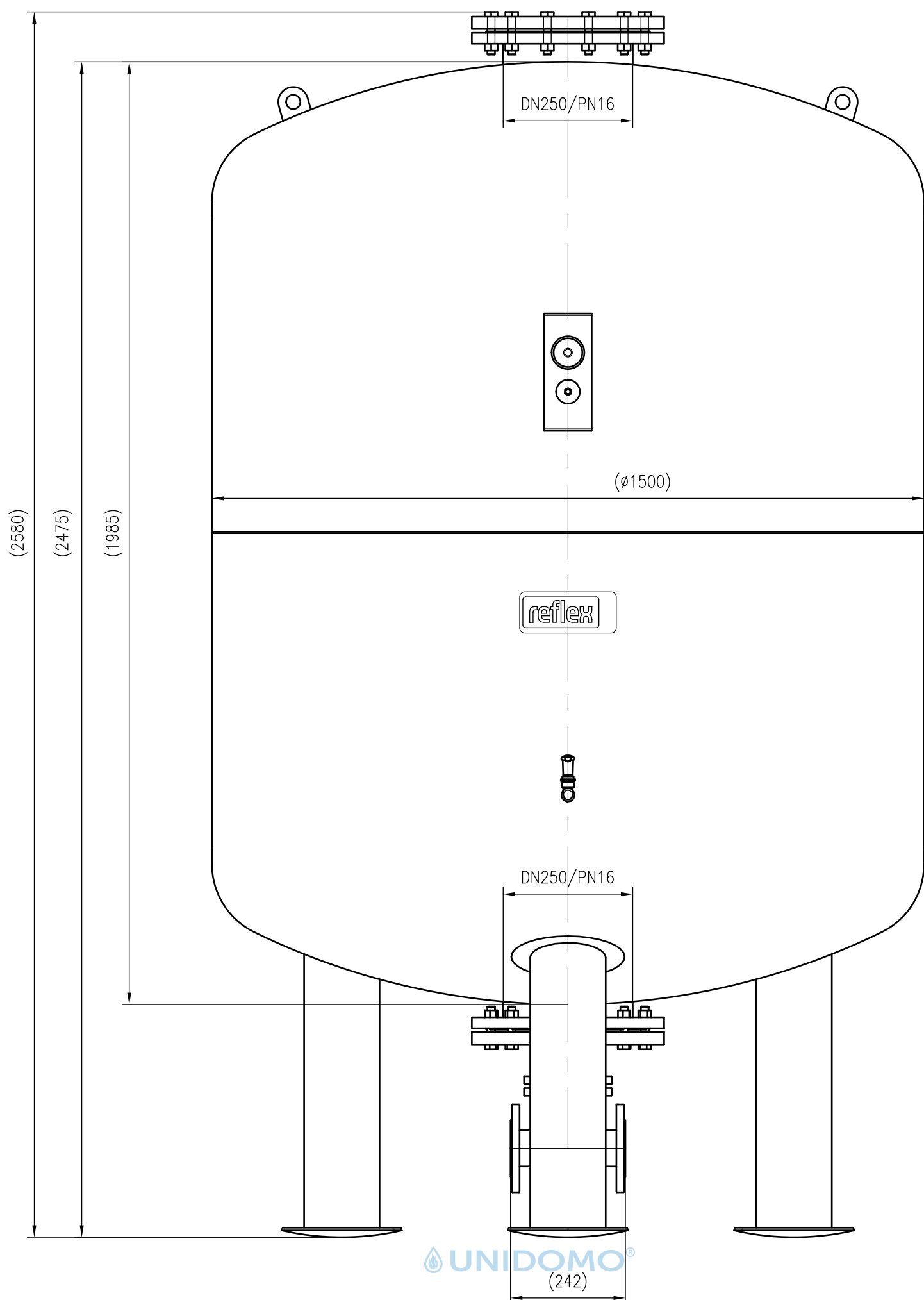
Front view
