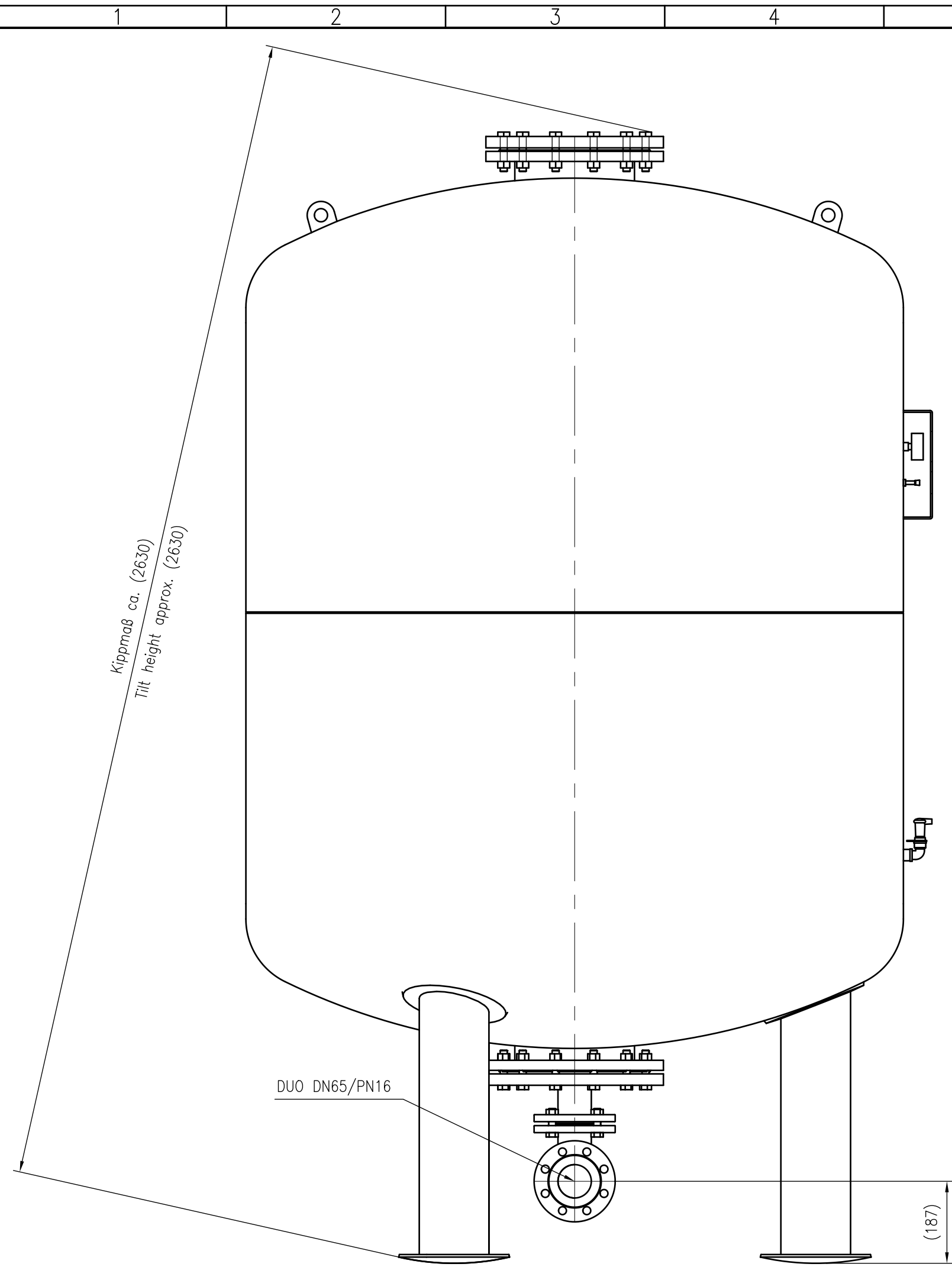
Side view
