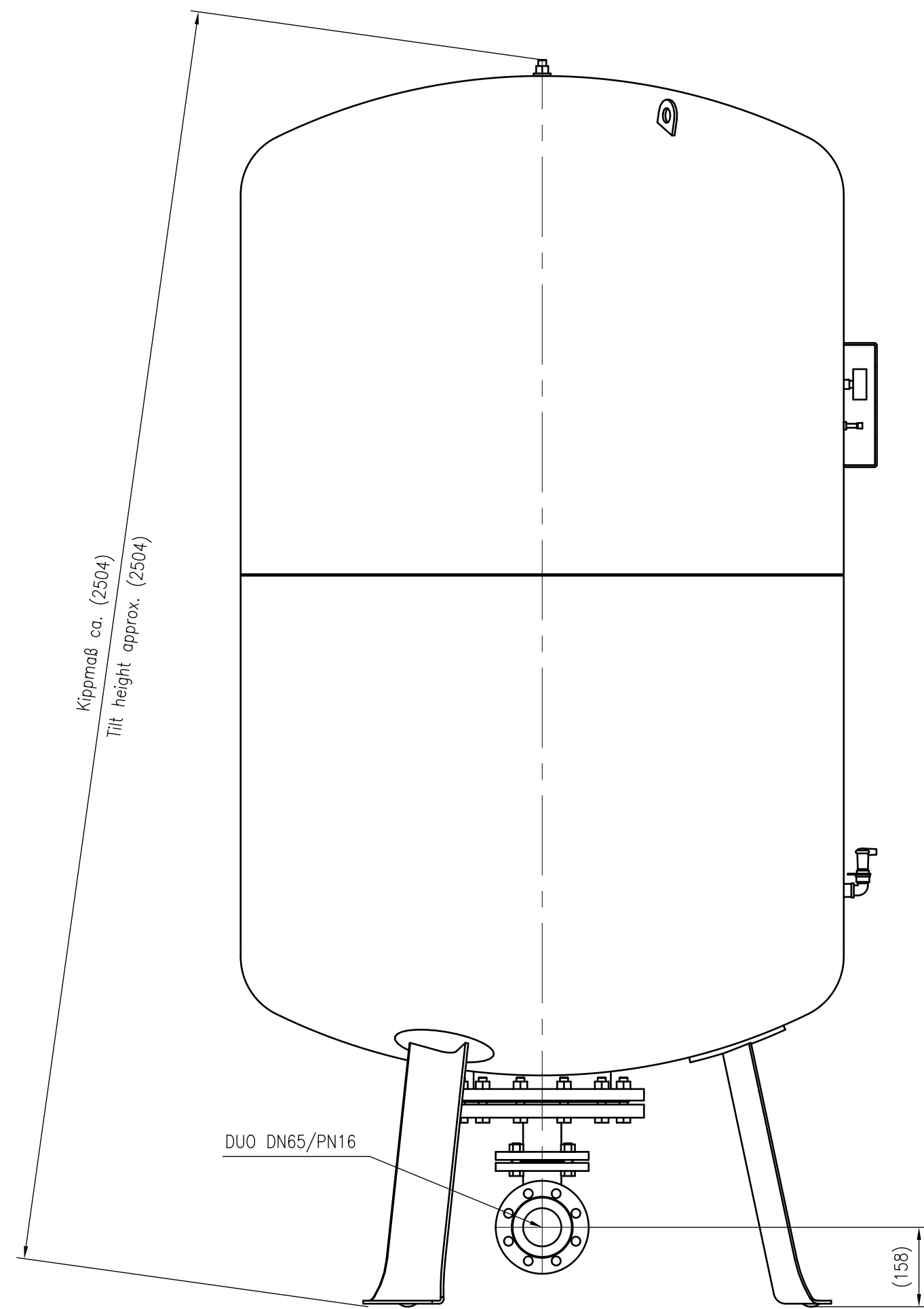
Side view
