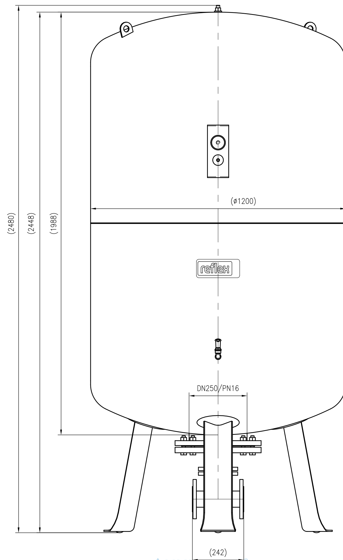
Front view
