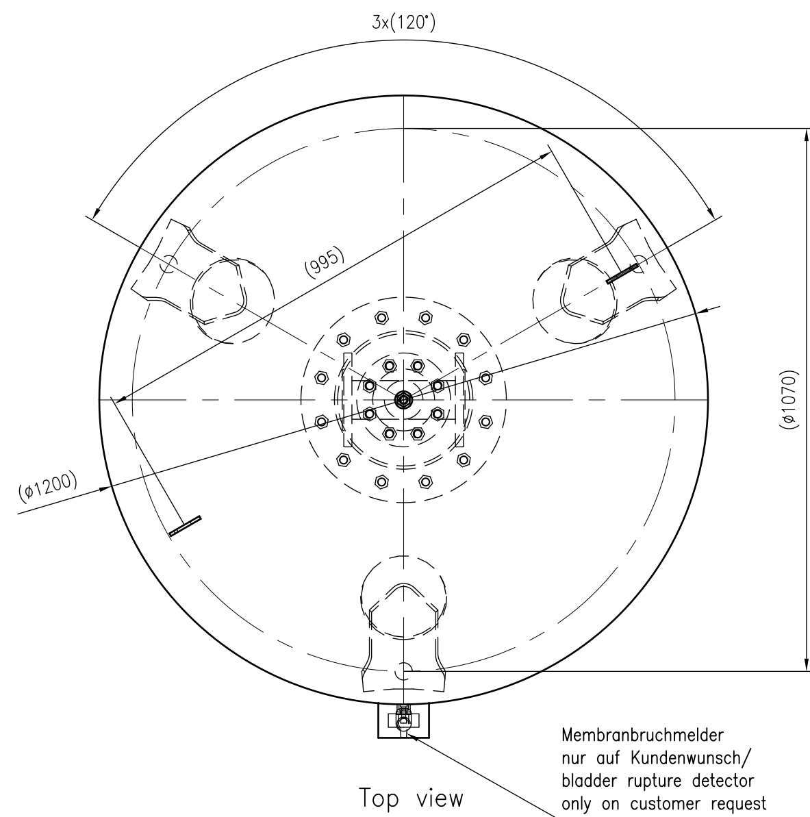
Top view
