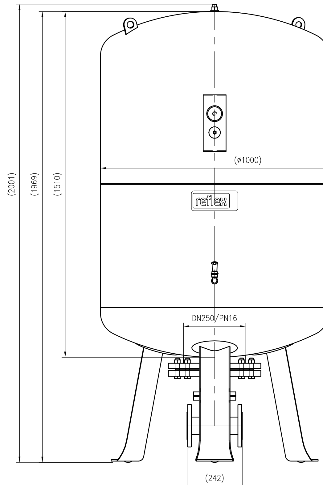
Front view
