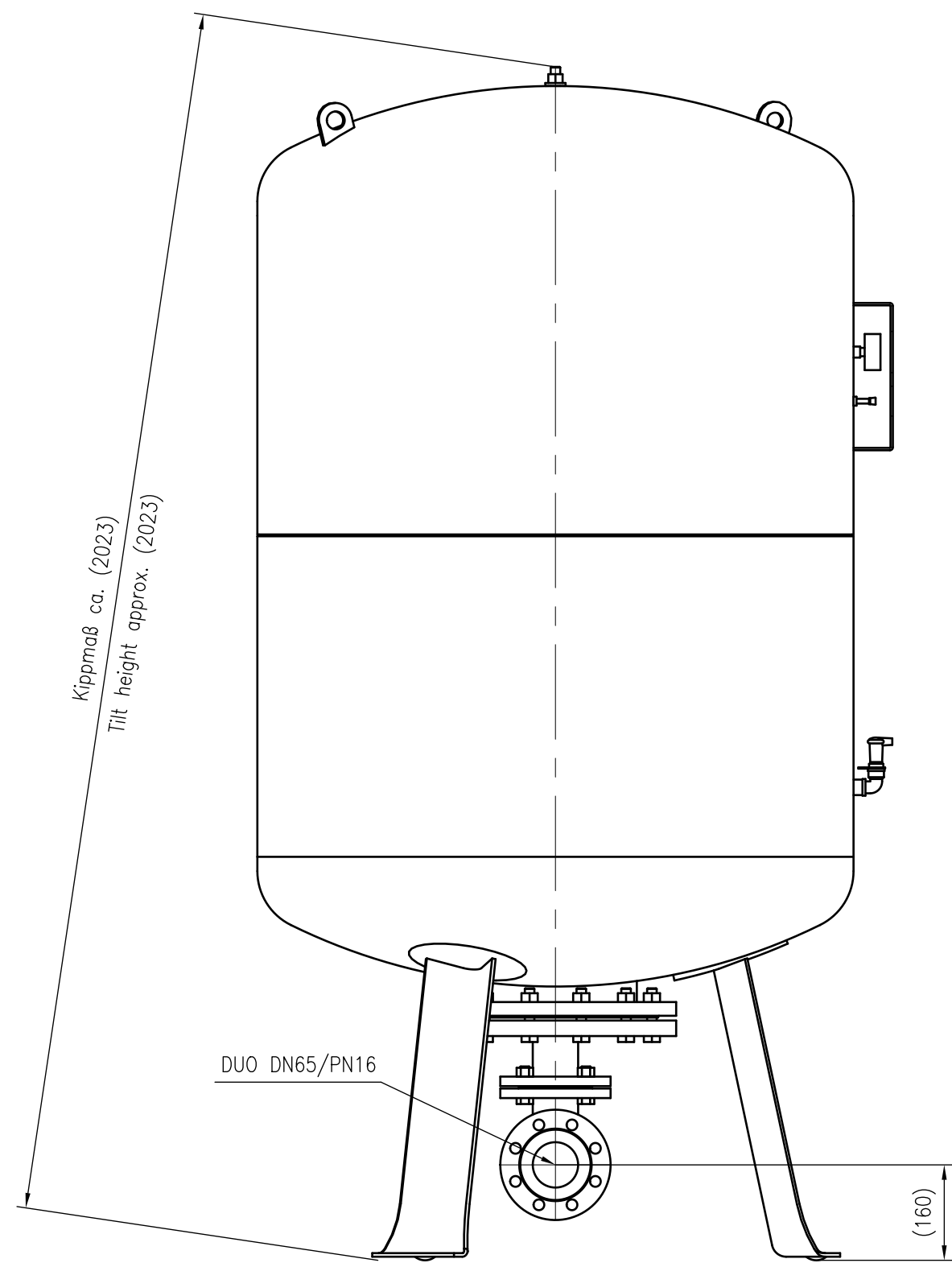
Side view
