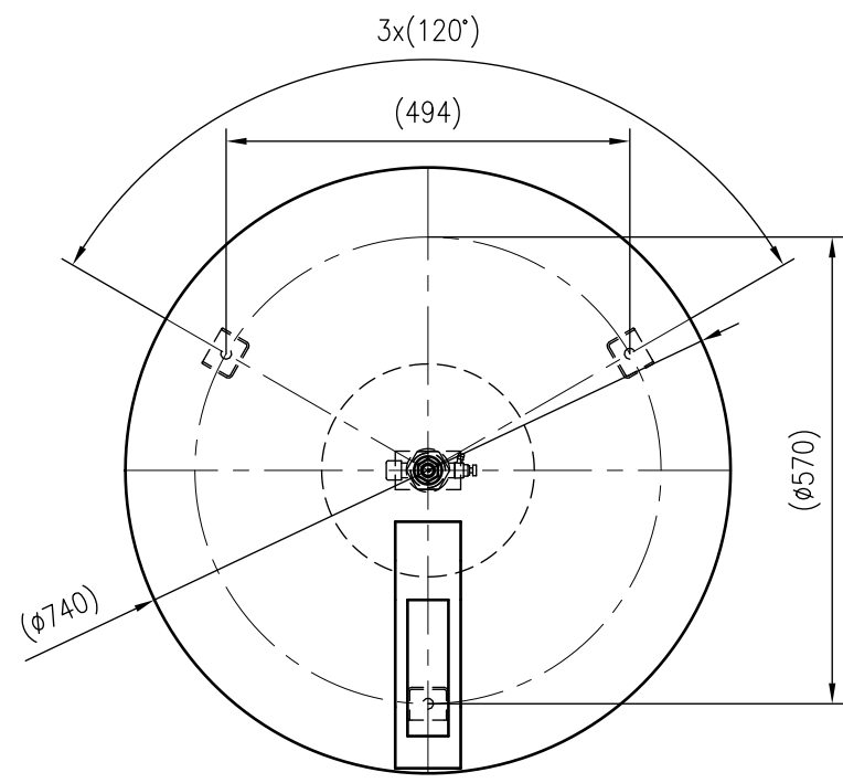
Top view
