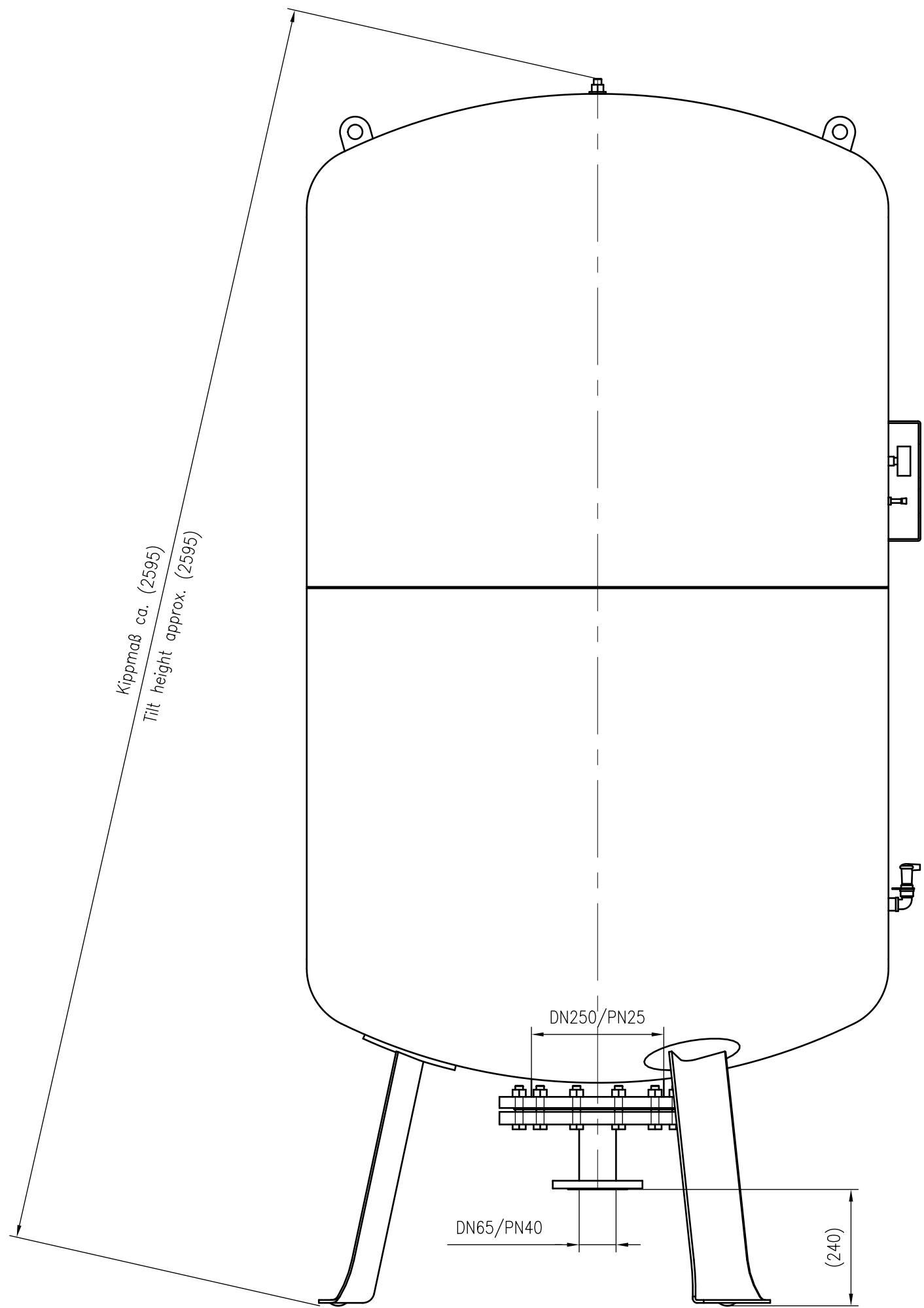
Side view
