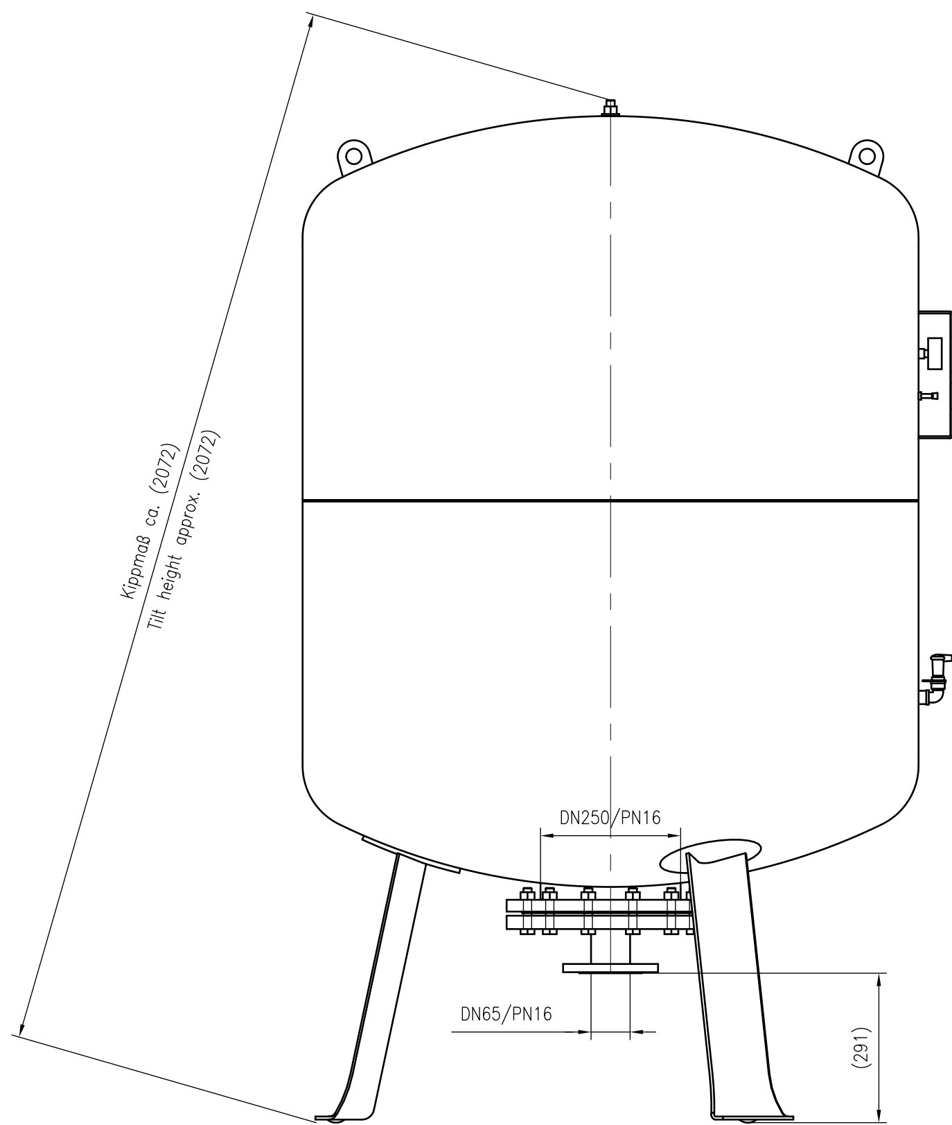
Side view
