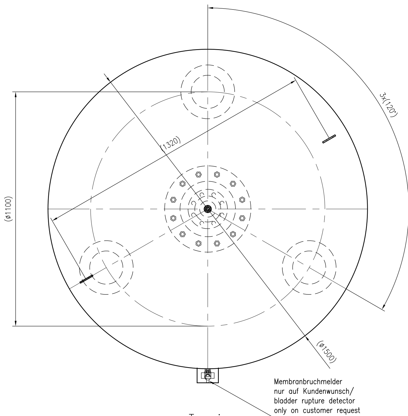
Top view
