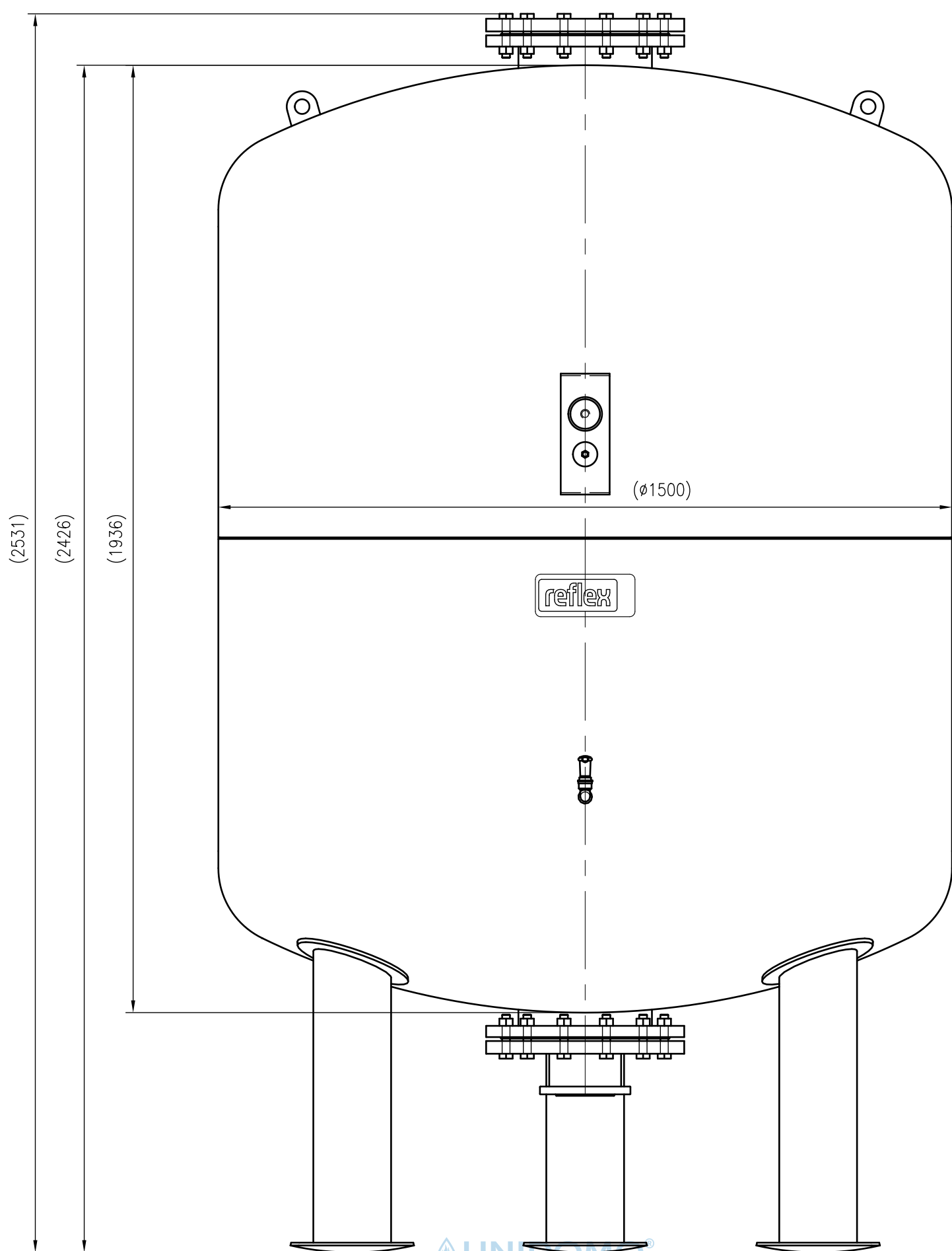
Front view
