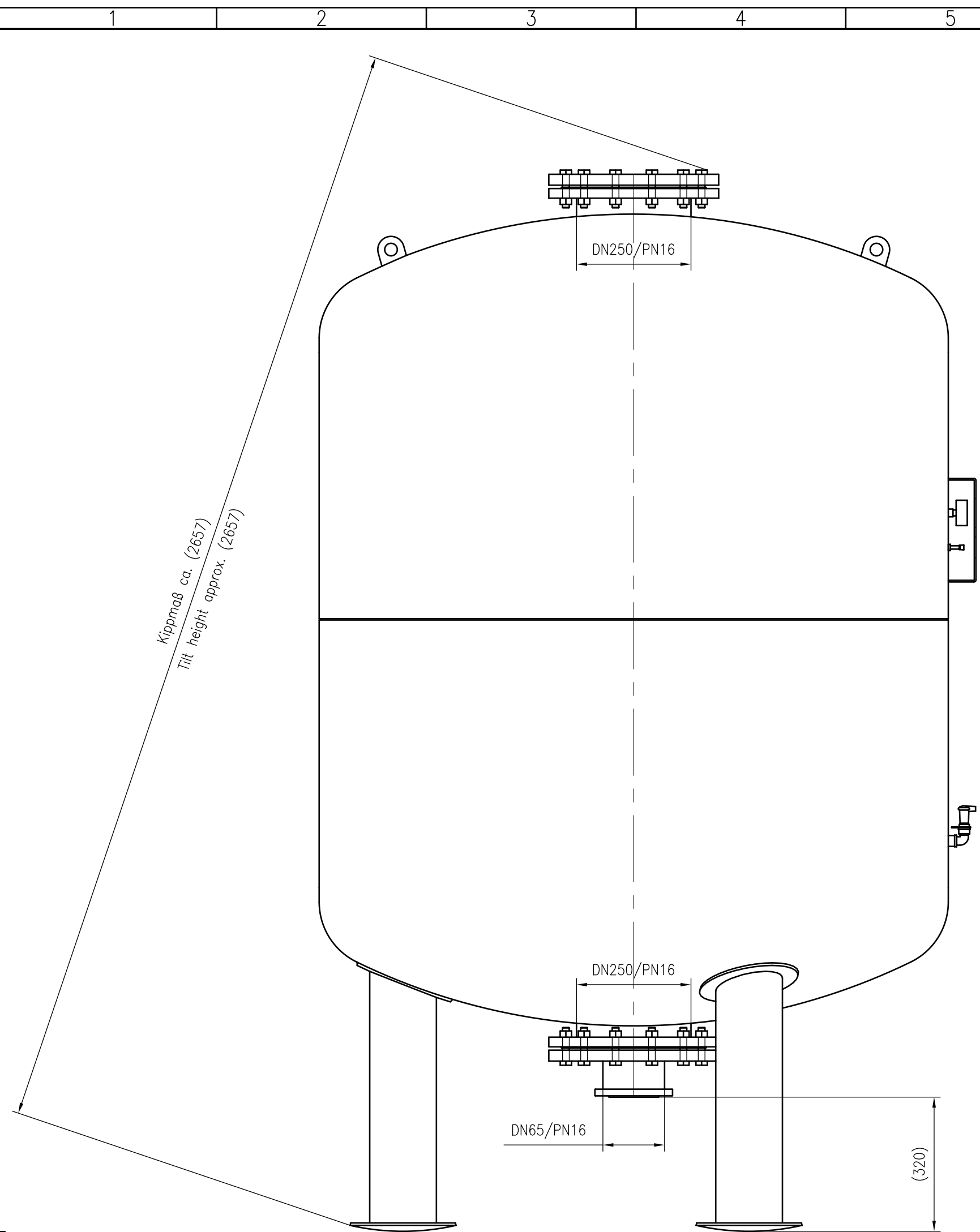
Side view
