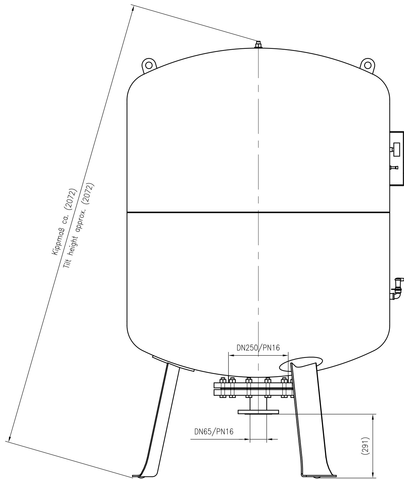
Side view
