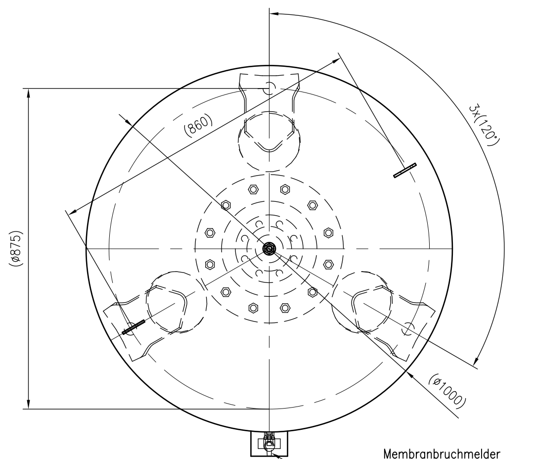
Top view
