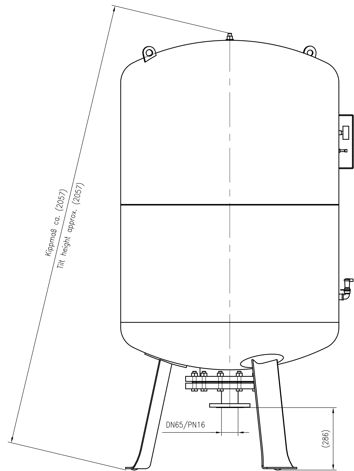
Side view
