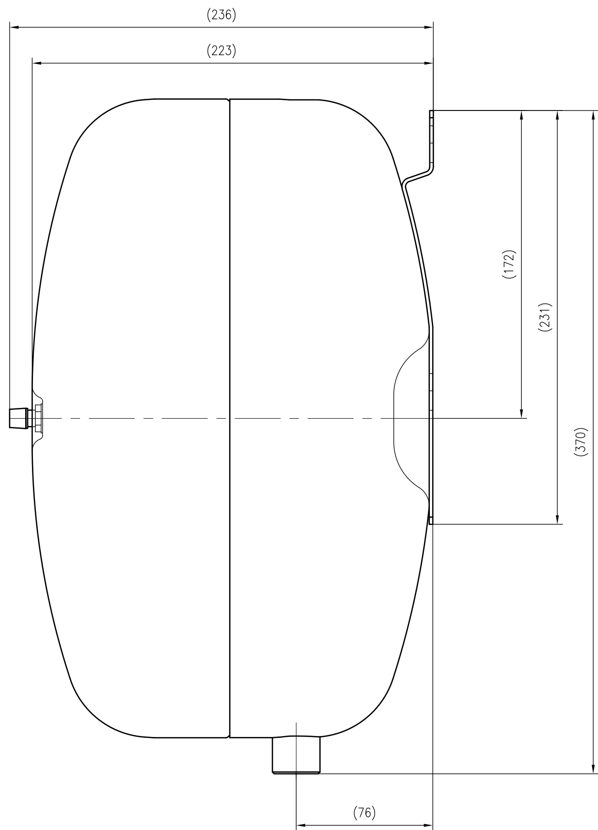
Side view
