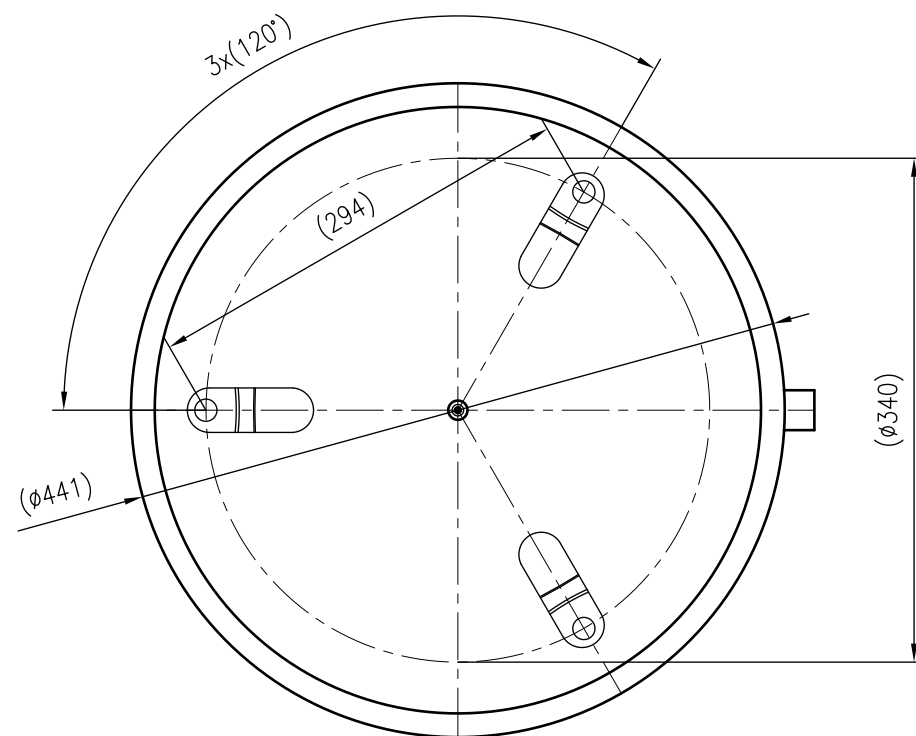
Top view
