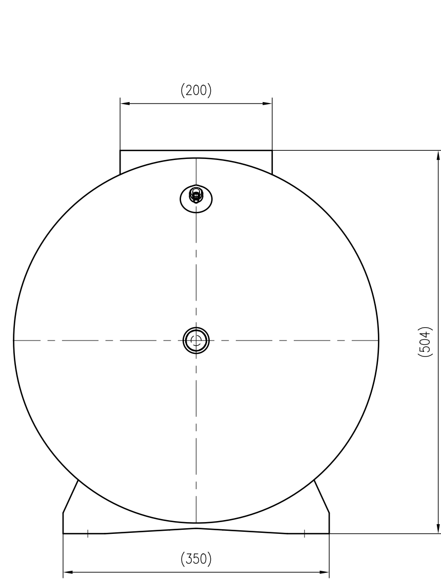
Side view
