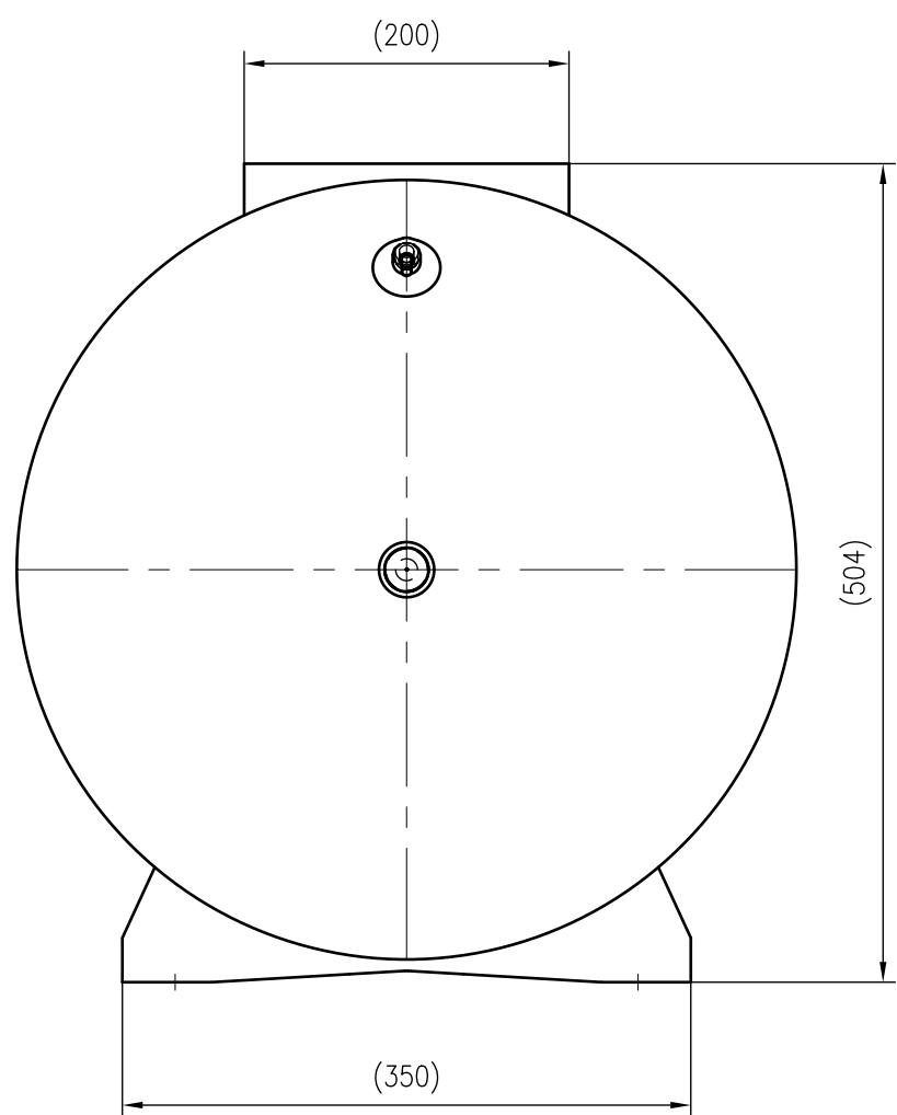
Side view
