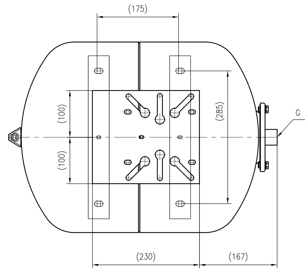
Top view
