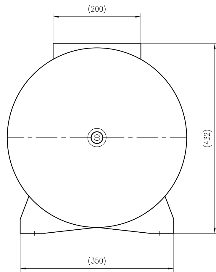
Side view
