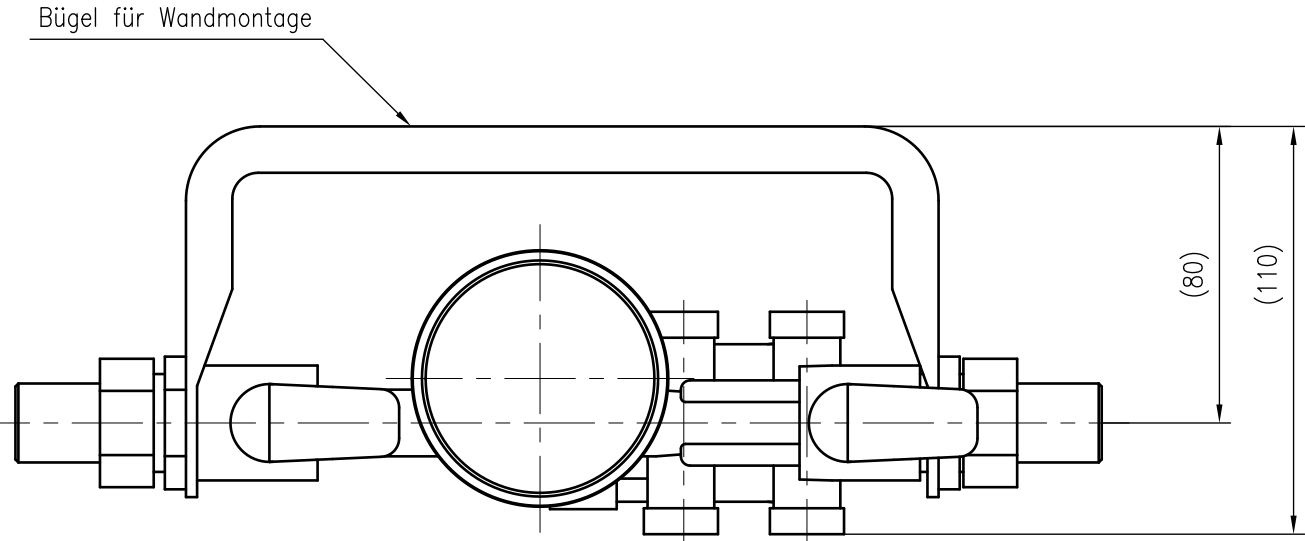
Top view
