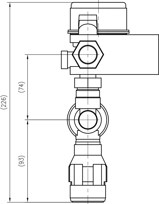
Side view
