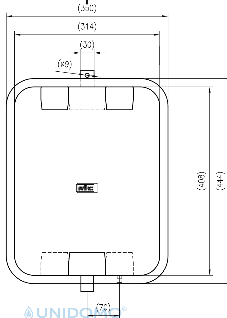
Front view
