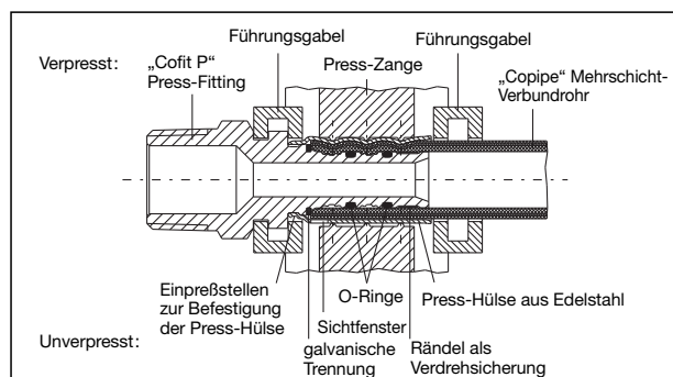
Oventrop Pressfitting
